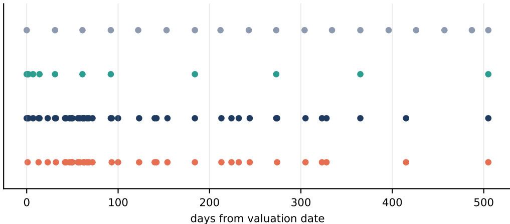
Simulation date grids: dense near term, sparse far term, event dates forced in
