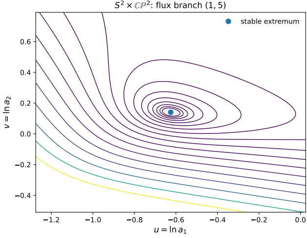
FIG. 2. Benchmark potential for the (1,5) branch. Although it has the same family index as (3,3), its flux distribution moves the minimum and changes the local Hessian.
