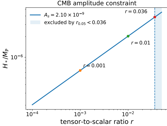
FIG. 3. The Hubble scale required by the measured scalar amplitude as a function of r . The shaded region is excluded by the current BICEP/Keck bound.
