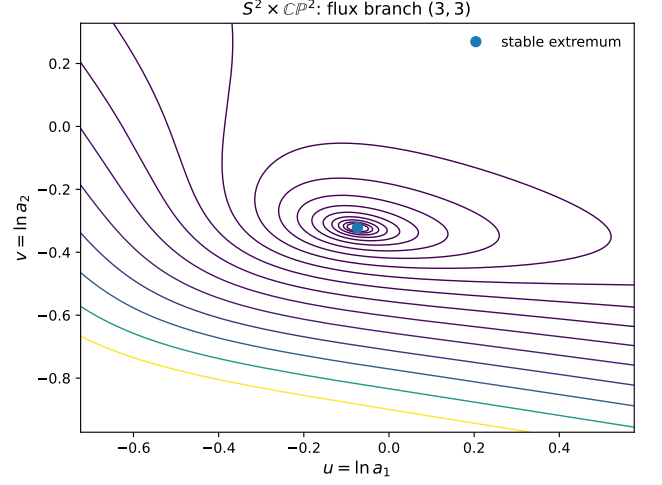
FIG. 1. Benchmark potential for the (3, 3) branch on S^2 \times \mathbb{CP}^2 . The dot marks the stable extremum.
