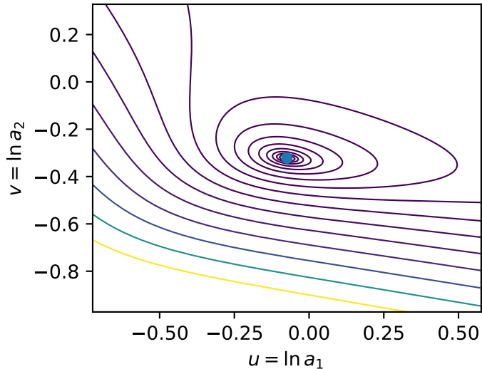
(3, 3) branch
