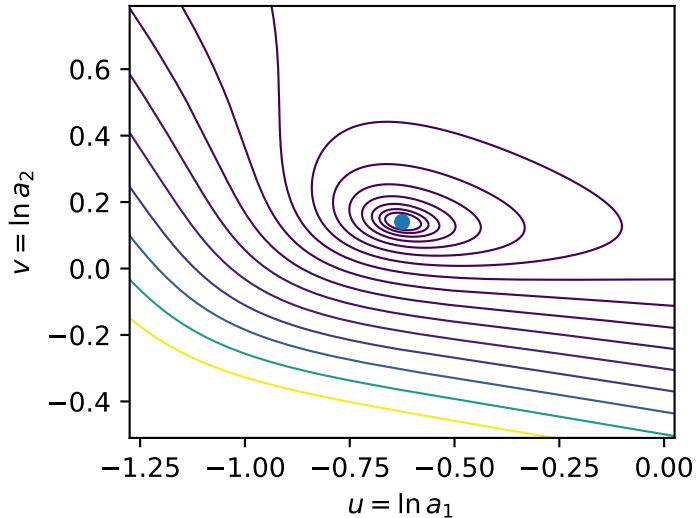
(1, 5) branch
