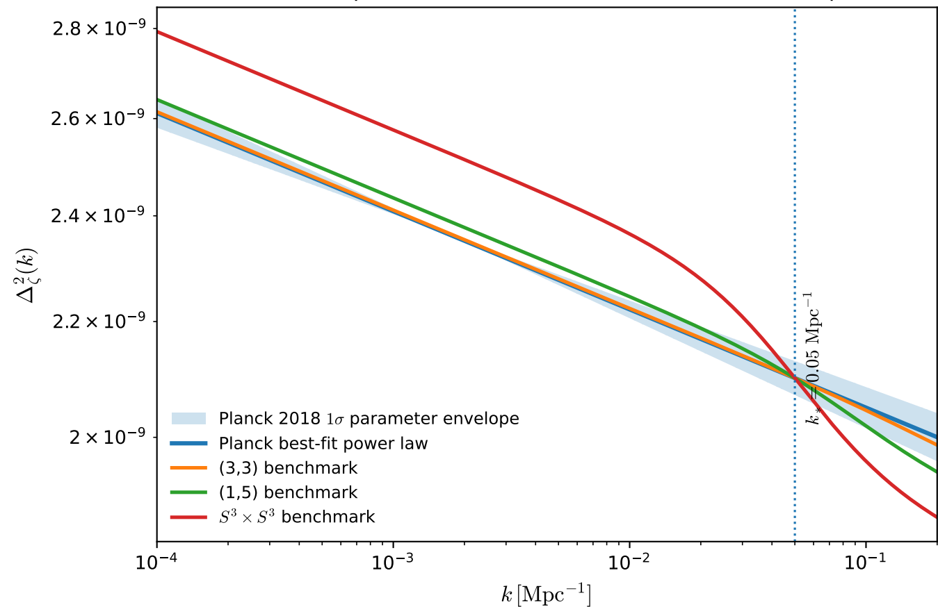
Benchmark compactifications versus the observed scalar spectrum
