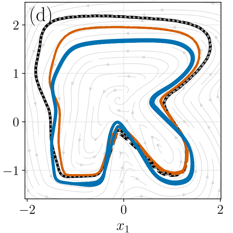
IROS: RShape
