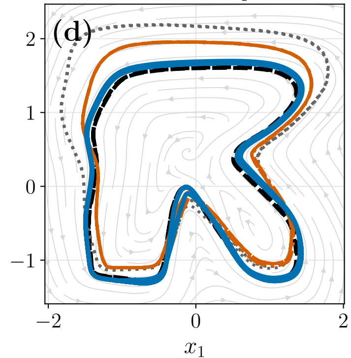
IROS: RShape
