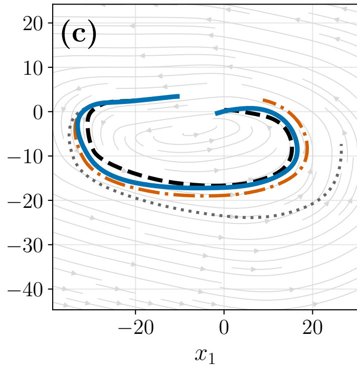
LASA: DoubleBendedLine
