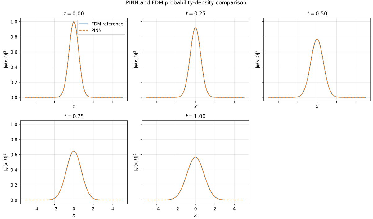
Figure 6: Comparison of the PINN and FDM probability-density profiles at selected time instants.
