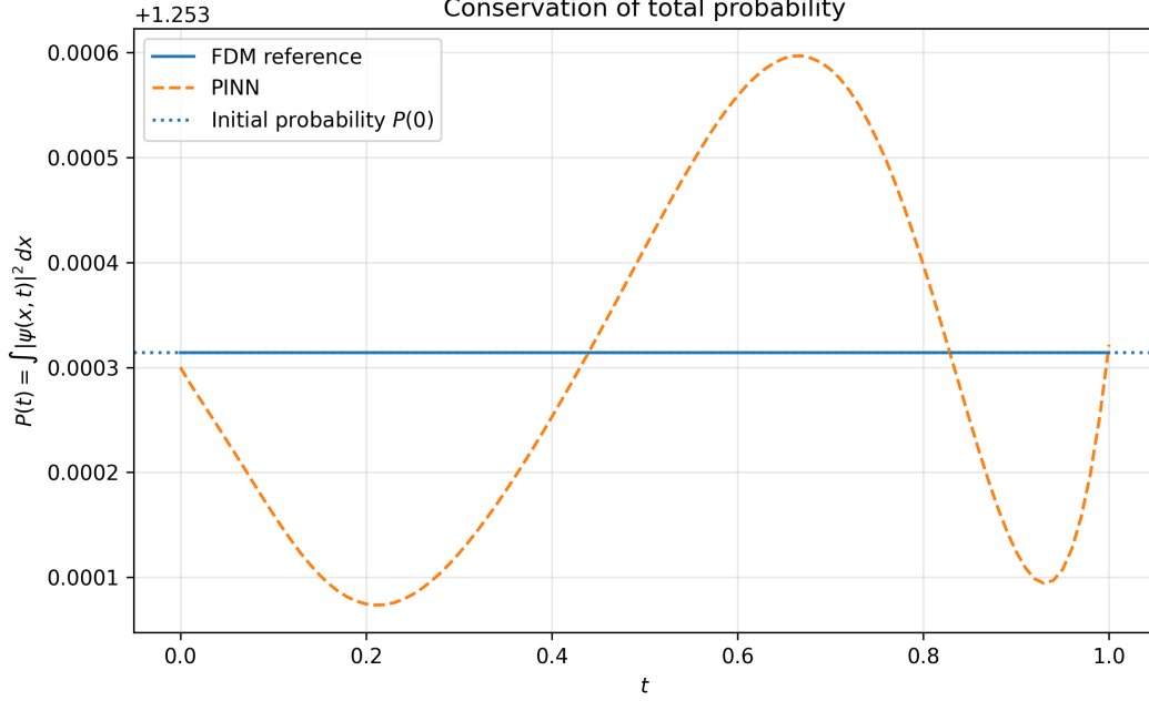
Figure 8: Temporal evolution of the wave-function norm obtained from the PINN and FDM solutions.
