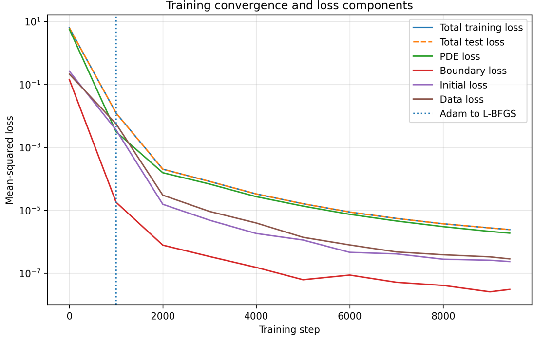
Figure 4: Convergence history of the total training and testing losses and the individual PINN loss components. The vertical dotted line indicates the transition from Adam to L-BFGS.
