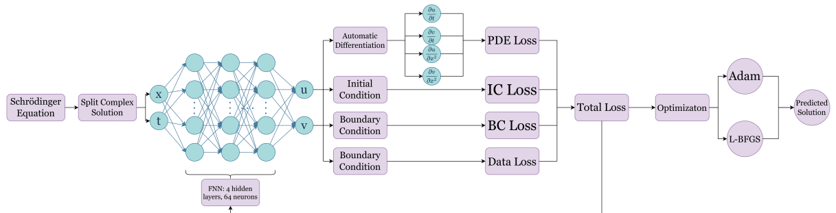
Figure 3: Diagram of solving Schrodinger with PINN
