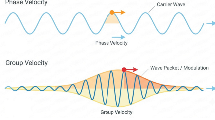
(a) Phase velocity vs Group velocity
