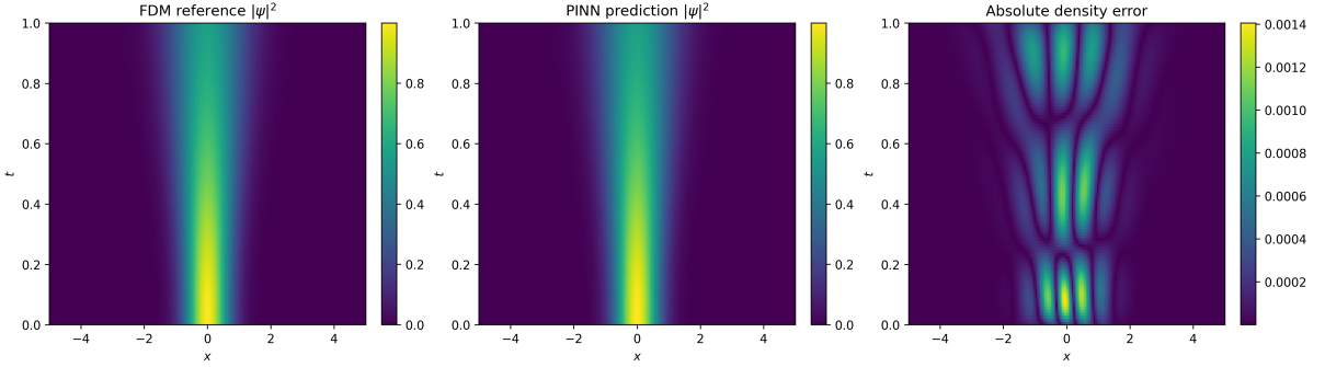
Figure 5: Comparison of the FDM reference probability density, the PINN prediction, and the pointwise absolute density error throughout the space-time domain.
