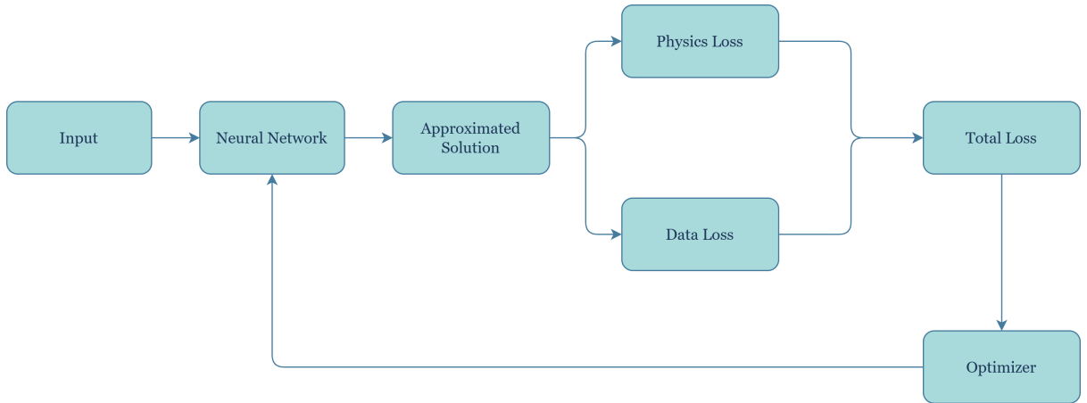
Figure 2: PINN Framework
