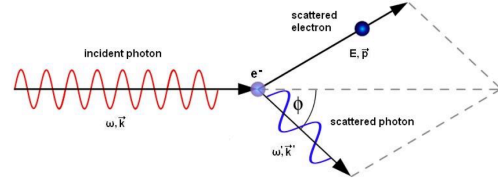
(b) Compton effect: scattering of a photon on a resting electron
