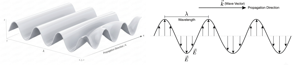
Figure 1: Plane waves in two and three dimensions
