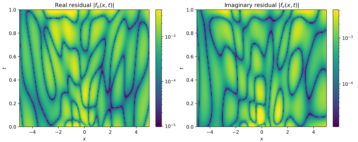
Figure 7: Absolute values of the real and imaginary Schrödinger equation residuals over the computational domain. A logarithmic colour scale is used to display the residual magnitudes.
