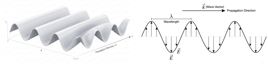
Figure 1: Plane waves in two and three dimensions
