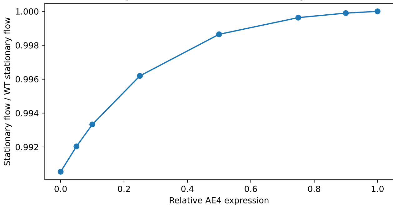
Stationary secretion on the full neutral charge manifold
