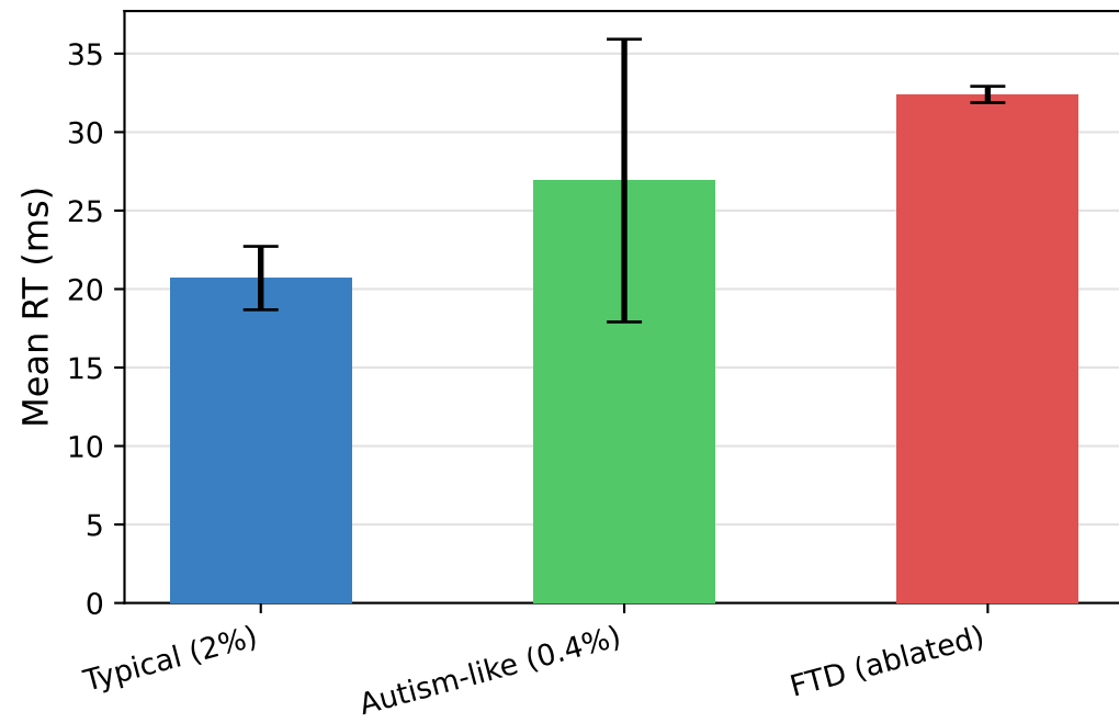
Clinical Conditions — Npyr=2000, 10 seeds, Fixed \theta=3
