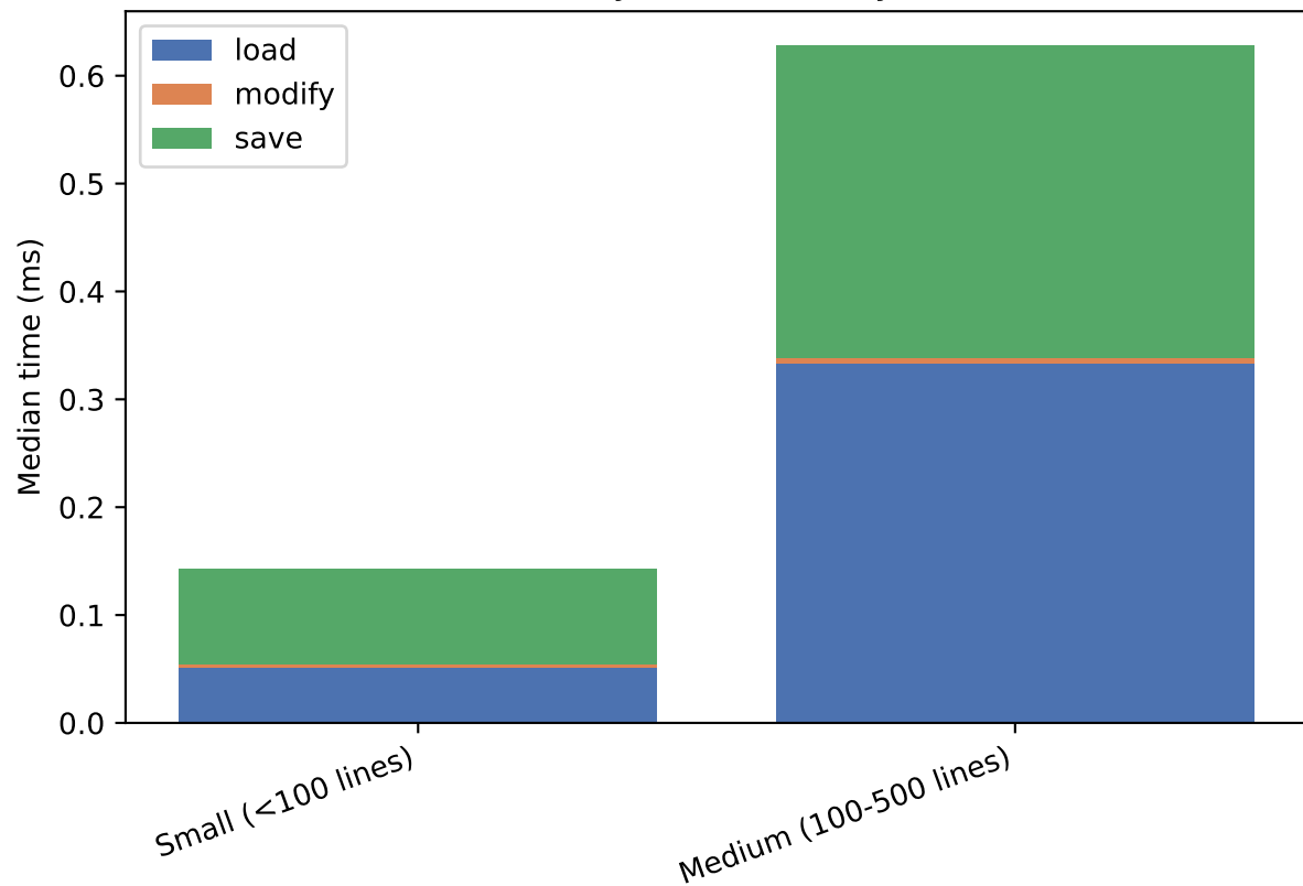
Median Load+Modify+Save time by file size bucket
