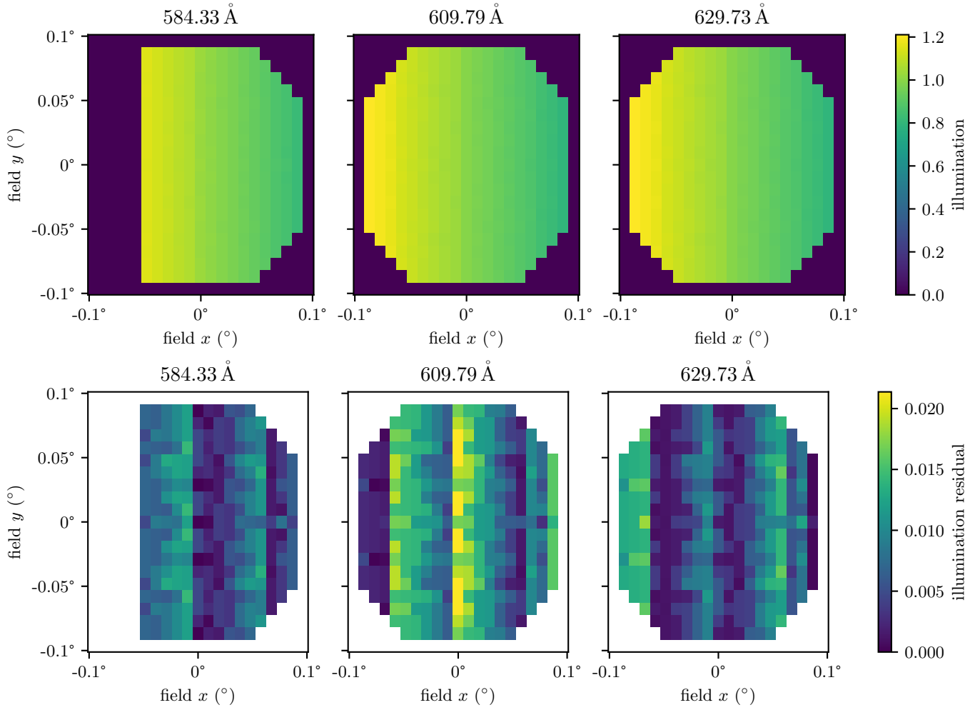
Figure 4. (Top) The relative illumination of a single ESIS channel as a function of position in the FOV, at each of the three target lines in the passband. The illumination is the fraction of the pupil which is unvignetted, normalized so that its average over the FOV is unity. (Bottom) The residual between that illumination and a linear model of it, plotted only where the model was fit.
