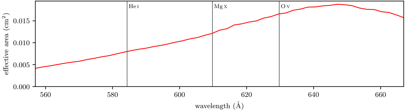
Figure 3. The effective area of a single ESIS channel over its passband, with the emission lines carried by the instrument model marked where they fall. The spectrum of the ?? brightest lines in the passband is still owed.
