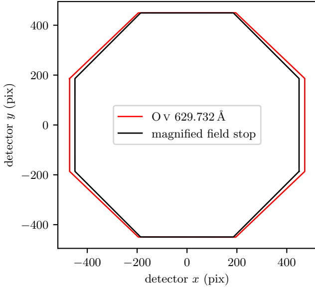
Figure 5. Plot of the magnified, undistorted field stop aperture vs. the distorted O v 629.732 Å image of the field stop aperture on the ESIS detector. The magnification factor used for the undistorted field stop aperture is the ratio of the grating exit arm to the grating entrance arm (4.01). The distorted image of the field stop aperture was calculated using the ESIS distortion model, described in Table 2.
