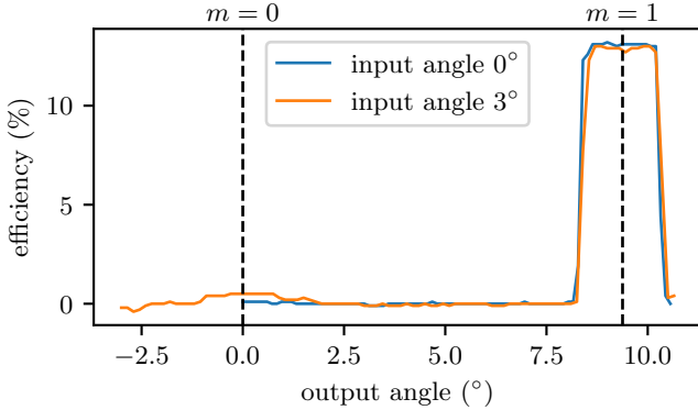
Figure 7. Measured efficiency at 63 nm of the Channel 2 grating as a function of reflection angle on 2018 January 21. Note flat response in first order over instrument FOV and suppression of zero order.
