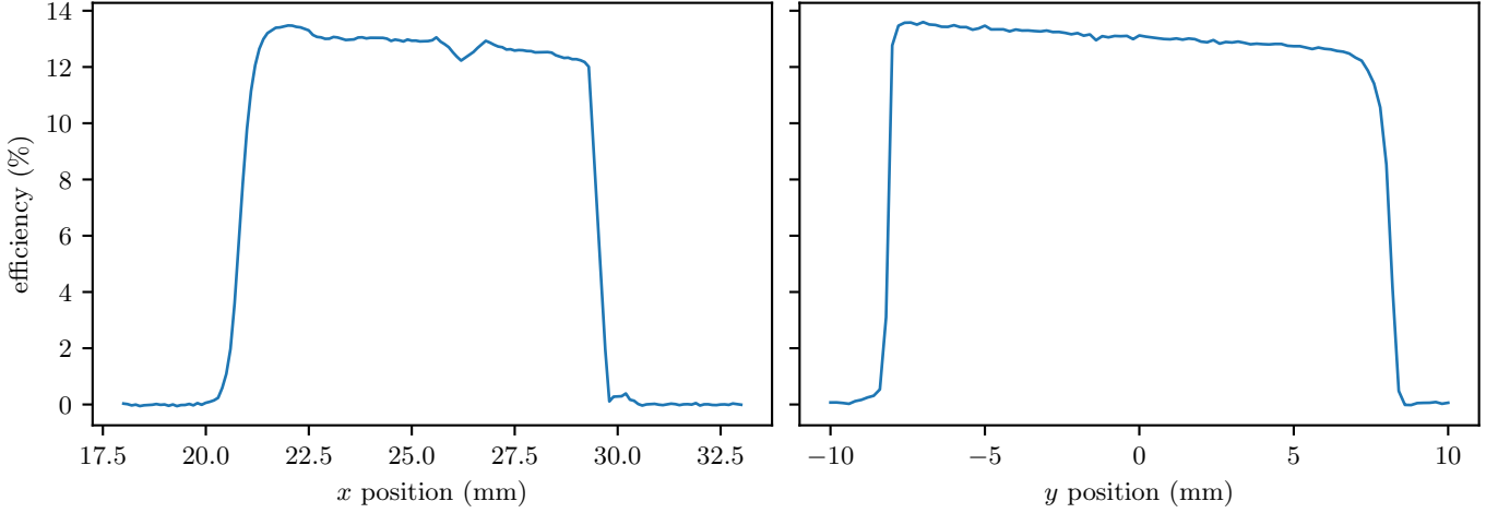
Figure 10. Channel 2 grating efficiency at 63 nm vs. position for two orthogonal slices across the optical surface on 2018 January 21.
