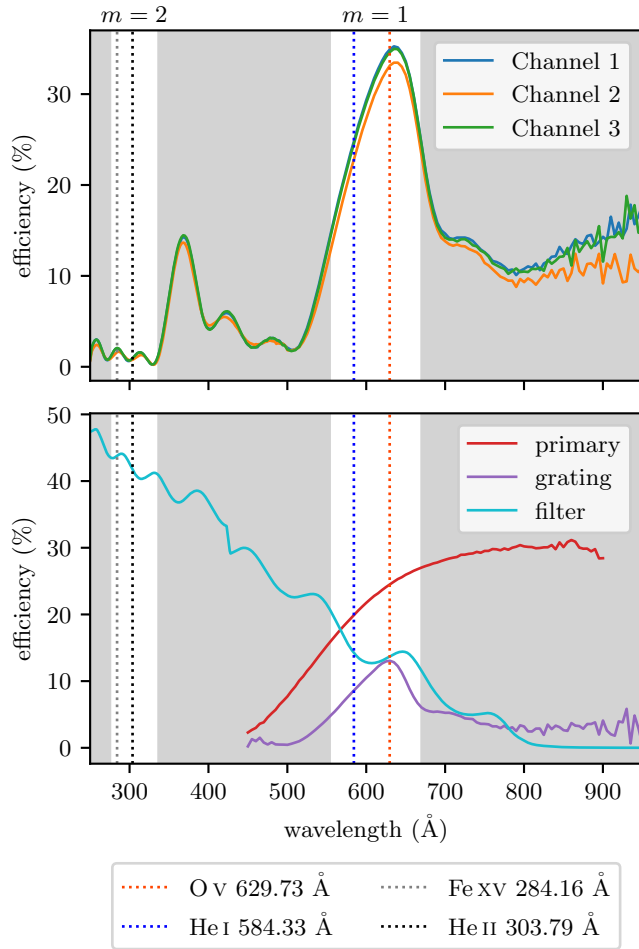
Figure 9. (Top) Measured reflectance for several multi-layer coated witness samples at an incidence angle of 4^\circ on 2018 January 21. The white regions indicate wavelengths that intercept the detector and the gray regions indicate wavelengths that miss the detector. Note the suppression of second order relative to the first order and the consistency of the coatings between each channel. The Channel 4 grating measurement is missing due to issues in the measurement apparatus. (Bottom) Comparison of the efficiency of the three main ESIS optical components: primary mirror, grating and filter. The primary mirror efficiency is based on measurements of a Si witness sample taken on 2018 May 10 at an angle of incidence of 4^\circ . The grating efficiency is from a measurement of the Channel 2 grating taken on 2018 January 21 at an angle of incidence of 0^\circ . The filter efficiency is a theoretical model that includes the filter mesh, 100 nm of Al and 4 nm of Al oxide.
