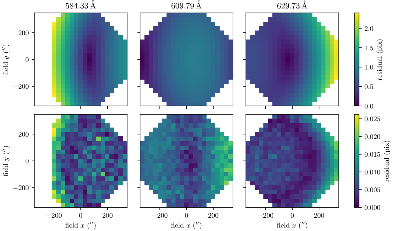
Figure 6. Magnitude of the residual between a linear distortion model and the raytrace model (top) and between a quadratic distortion model and the raytrace model (bottom). This figure demonstrates that a quadratic distortion model is sufficient to achieve sub-pixel accuracy.
