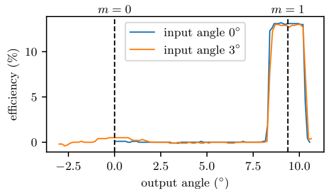
Figure 5. Measured efficiency at 63 nm of the Channel 2 grating as a function of reflection angle on 2018 January 21. Note flat response in first order over instrument FOV and suppression of zero order.
