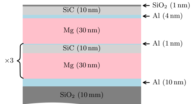
Figure 6. Schematic of the Al/SiC/Mg multilayer with N = 4 layers.
