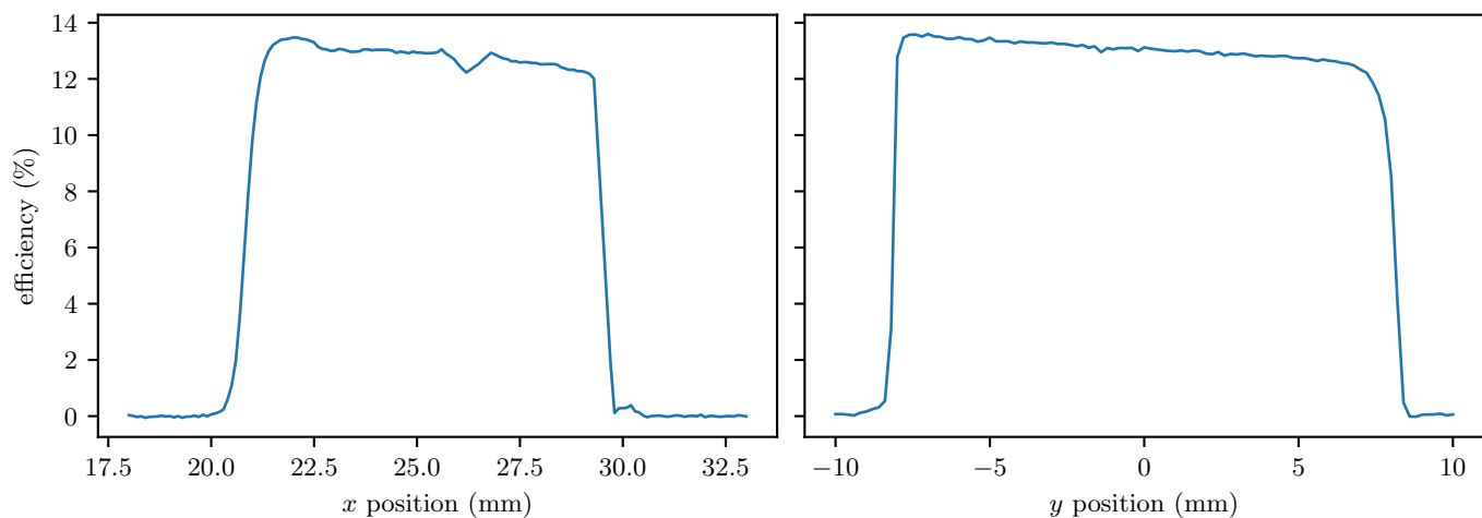
Figure 8. Channel 2 grating efficiency at 63 nm vs. position for two orthogonal slices across the optical surface on 2018 January 21.
