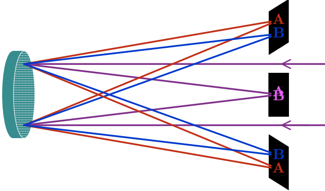
Figure 1. Schematic diagram of the MOSES instrument. Incident light from the right forms an undispersed image on the central m = 0 CCD. Dispersed images are formed on the outboard m = \pm 1 CCDs. The imaging of longer and shorter wavelengths is indicated by the use of red and blue letters respectively.
