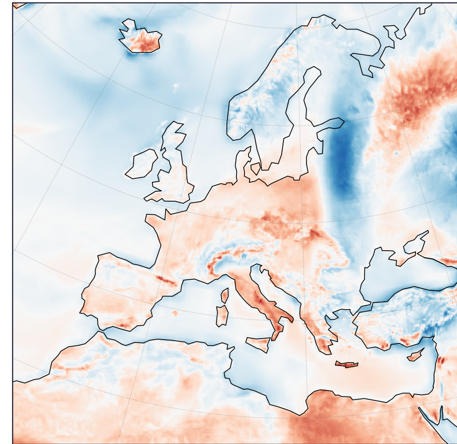
Residual (EC-Earth - HCLIM)
