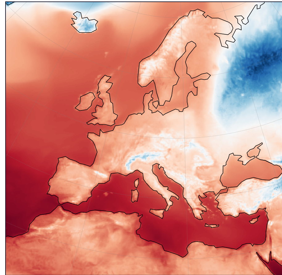
HCLIM
