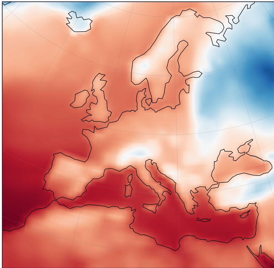
EC-Earth (regridded)
