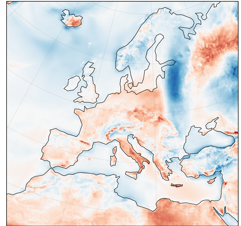
Residual (EC-Earth - HCLIM)
