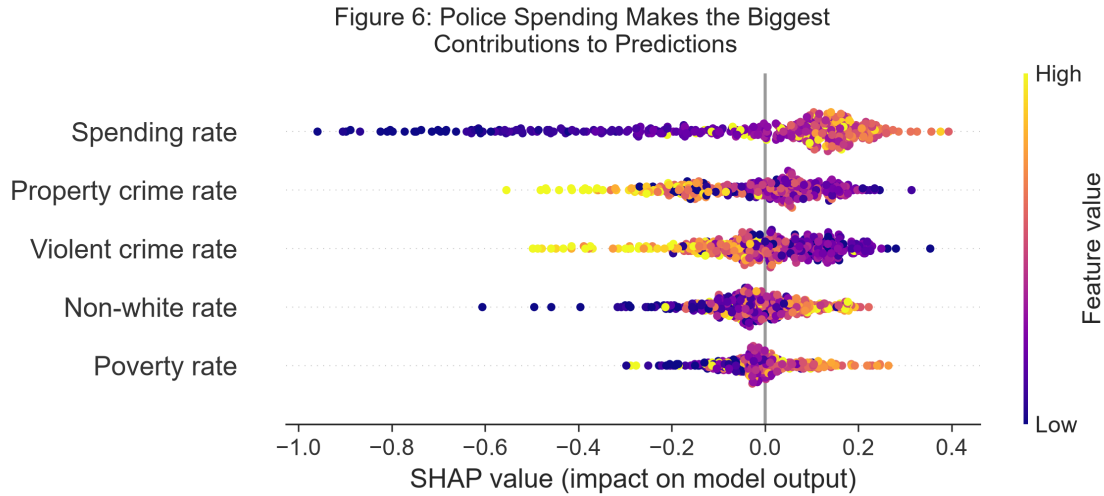
Figure 6: Figure 6: Graph displaying each instance of each feature, that instance's value by color, and how that instance impacted the mode's predictions.
