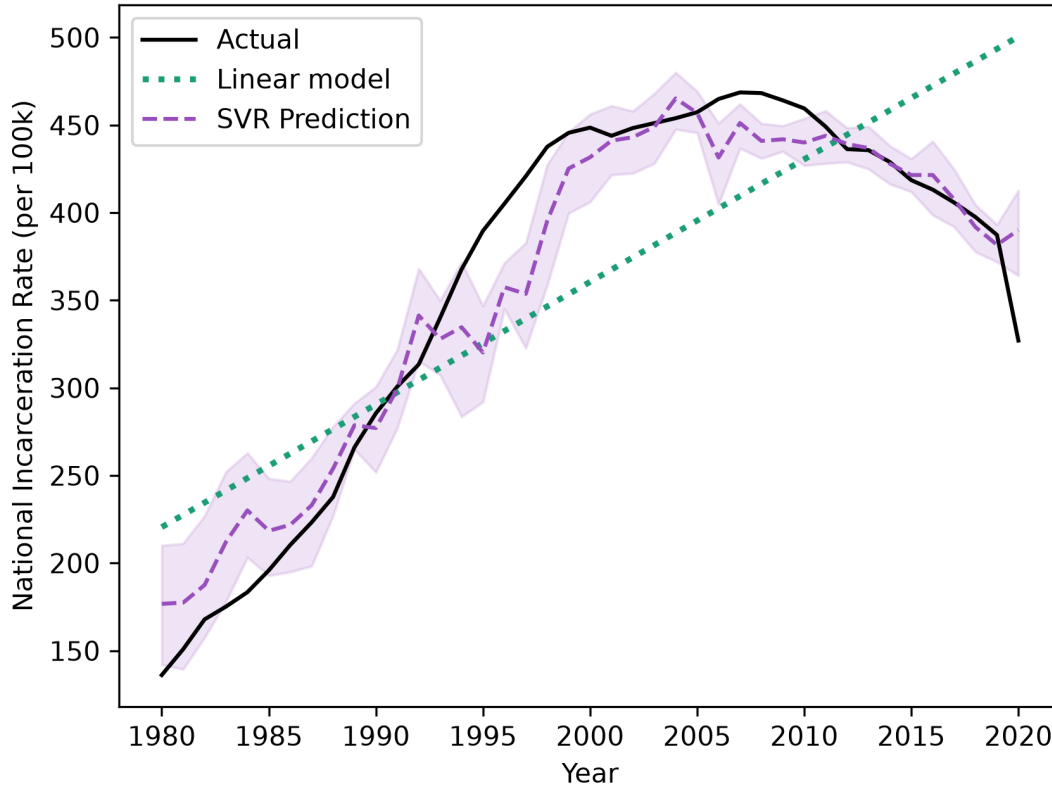
Figure 4: Predictions Made Using all Features are Much Closer to Reality
