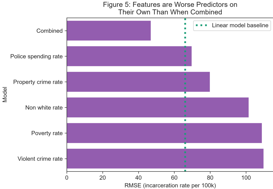
Figure 5: Figure 5: A barplot showing the RMSE of all models used in this project.
