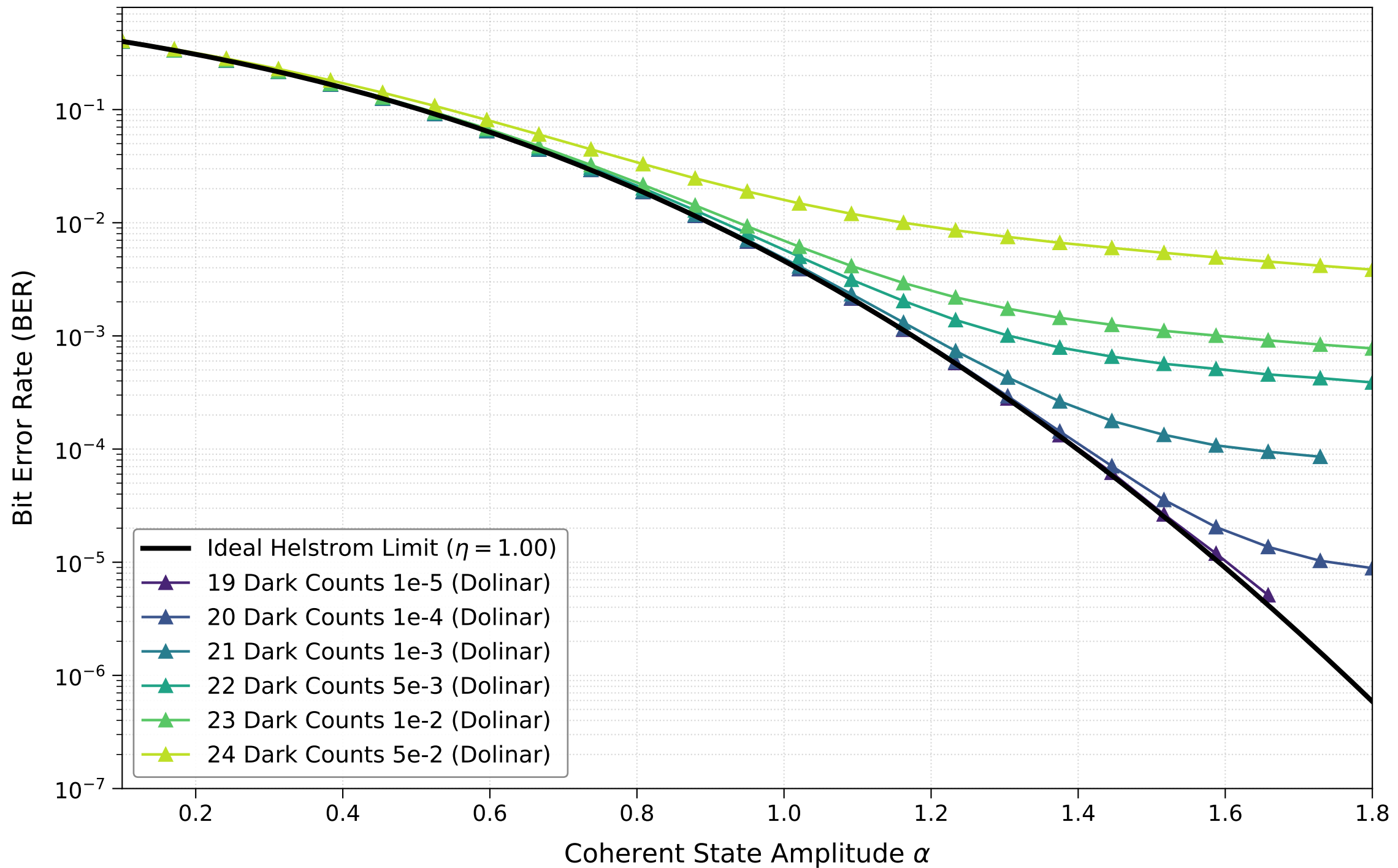
Impact of Dark Counts on Quantum Receiver Performance
