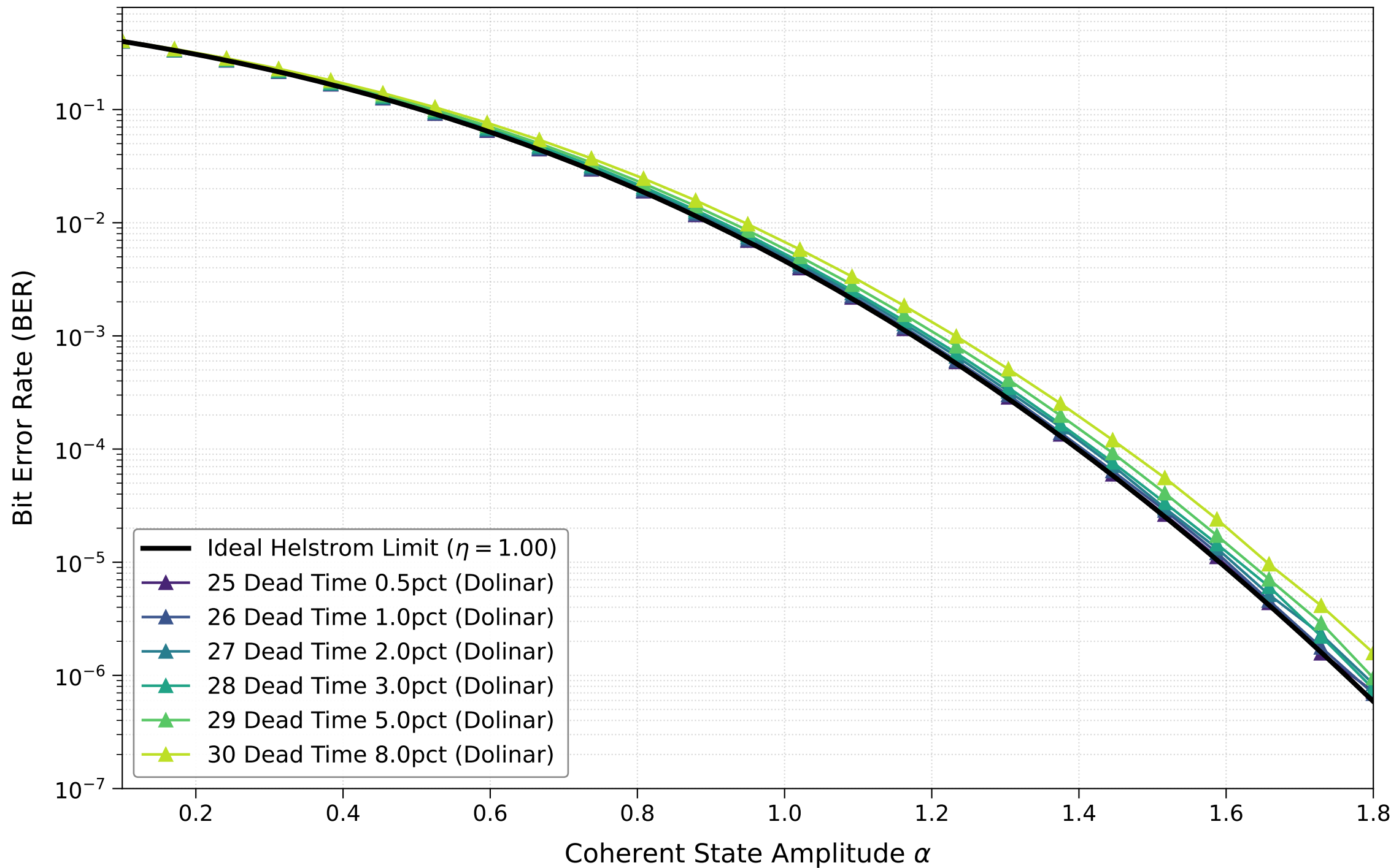
Impact of Dead Time on Quantum Receiver Performance
