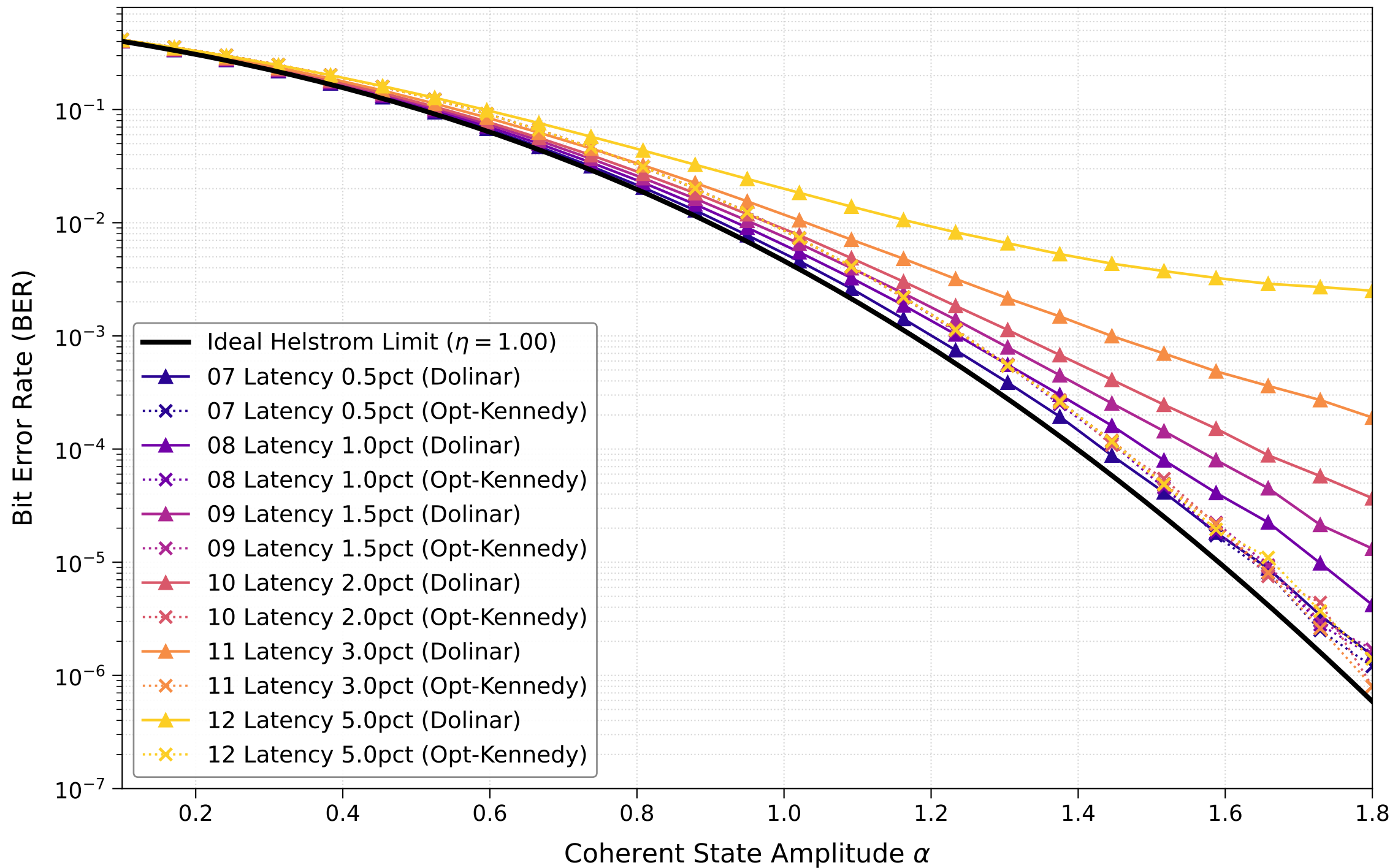
Impact of Latency on Quantum Receiver Performance
