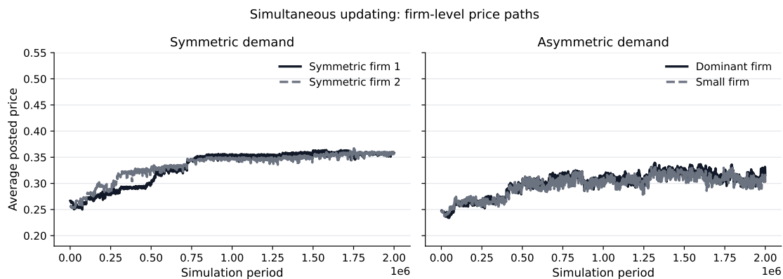
Figure A.3. FIRM-LEVEL PRICES UNDER SIMULTANEOUS UPDATING. The figure reports mean posted prices by firm under simultaneous updating. Within each run, prices are averaged over non-overlapping 1,000-period bins. The plotted series averages these bin-level prices across 30 runs.
