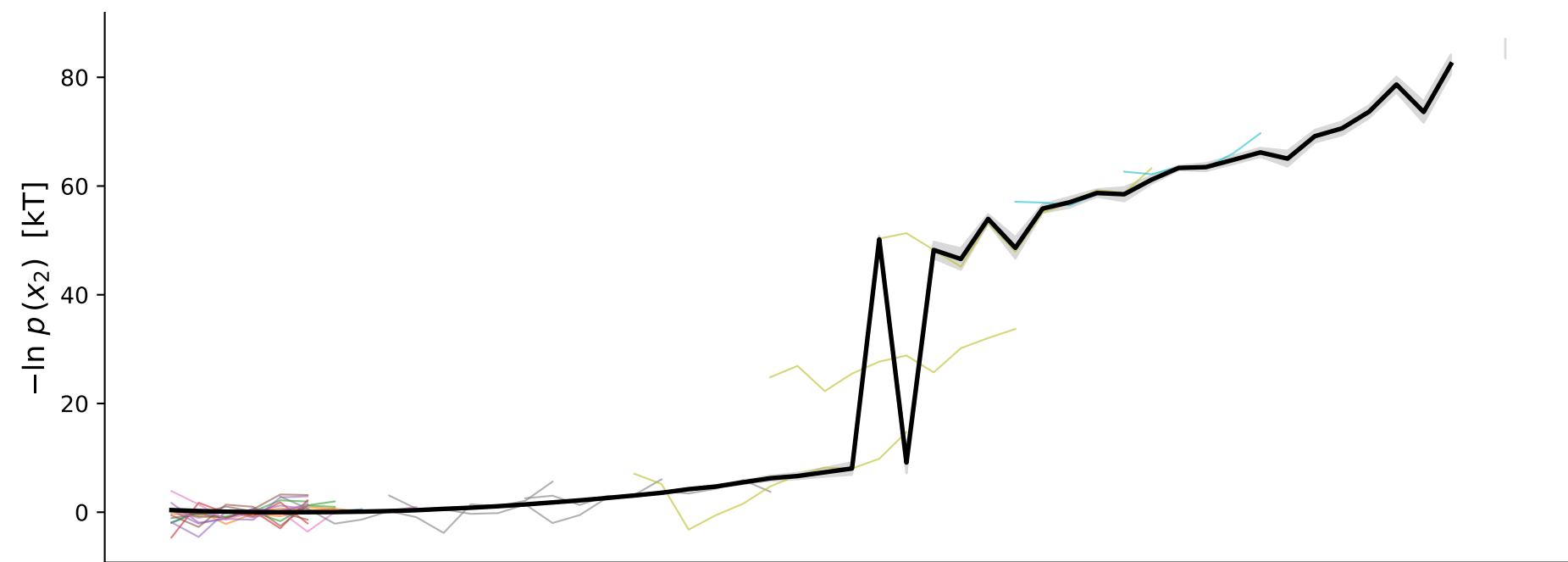
Biased histogram marginals along dimension 2
