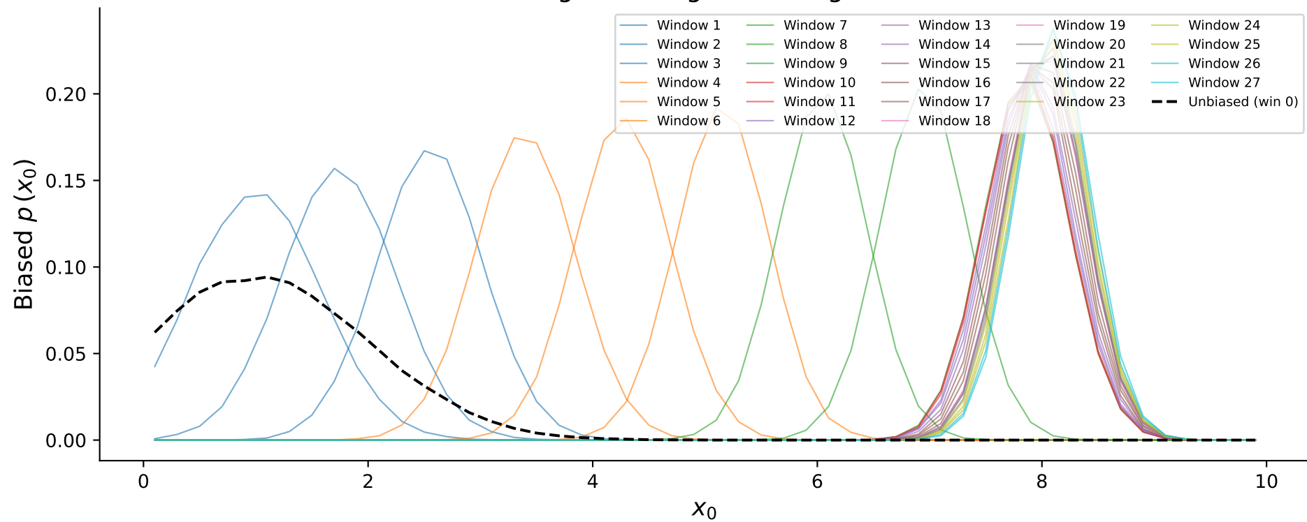
Biased histogram marginals along dimension 0
