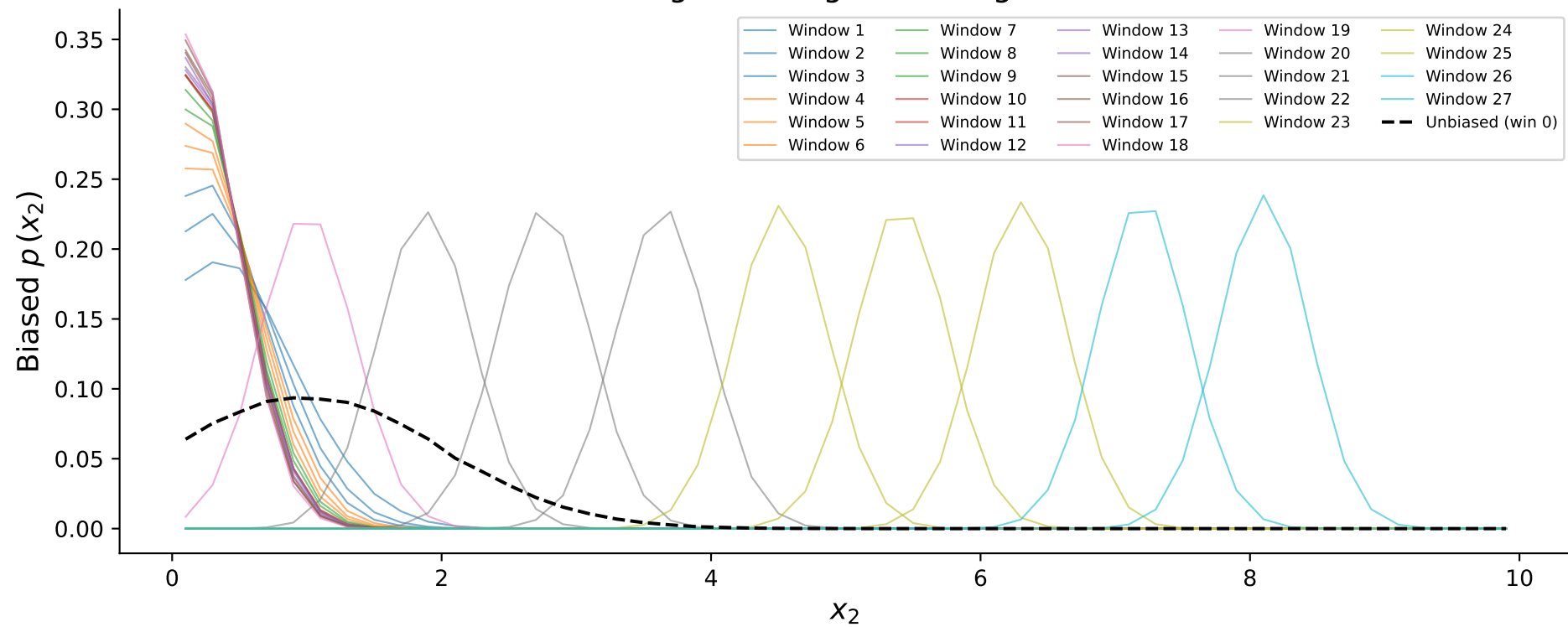
Biased histogram marginals along dimension 2
