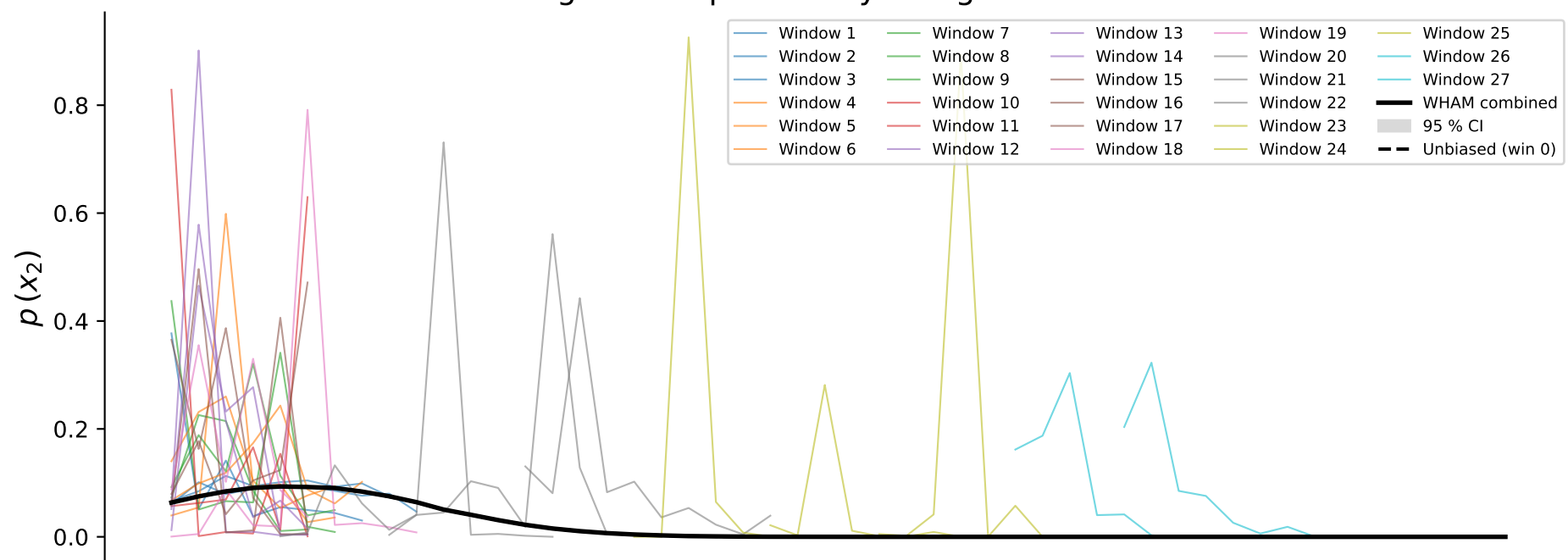
Marginalised probability along dimension 2
