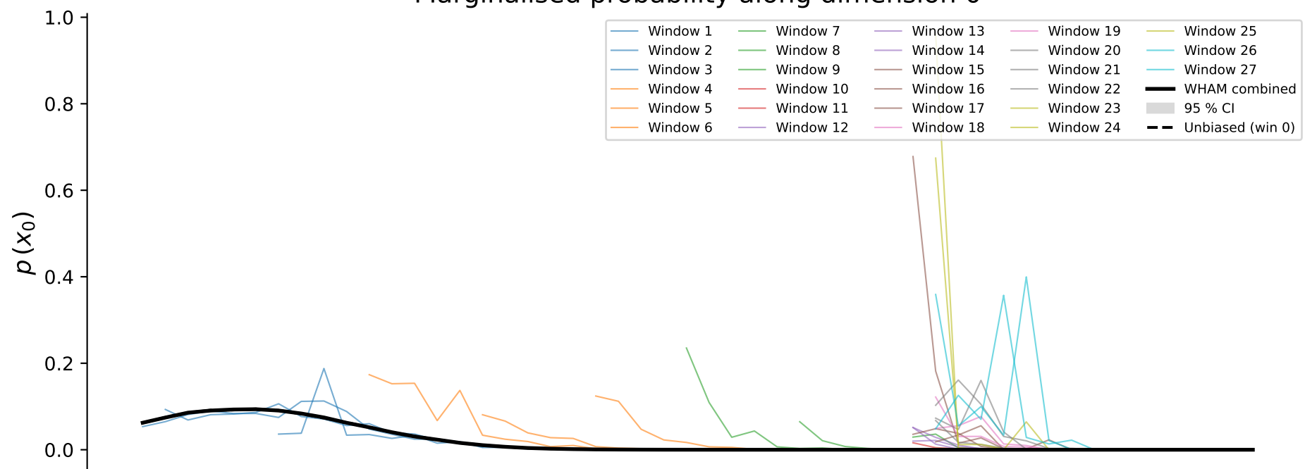
Marginalised probability along dimension 0
