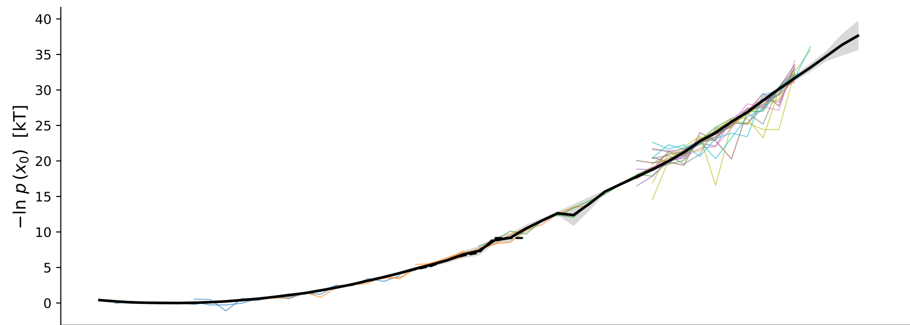
Biased histogram marginals along dimension 0
