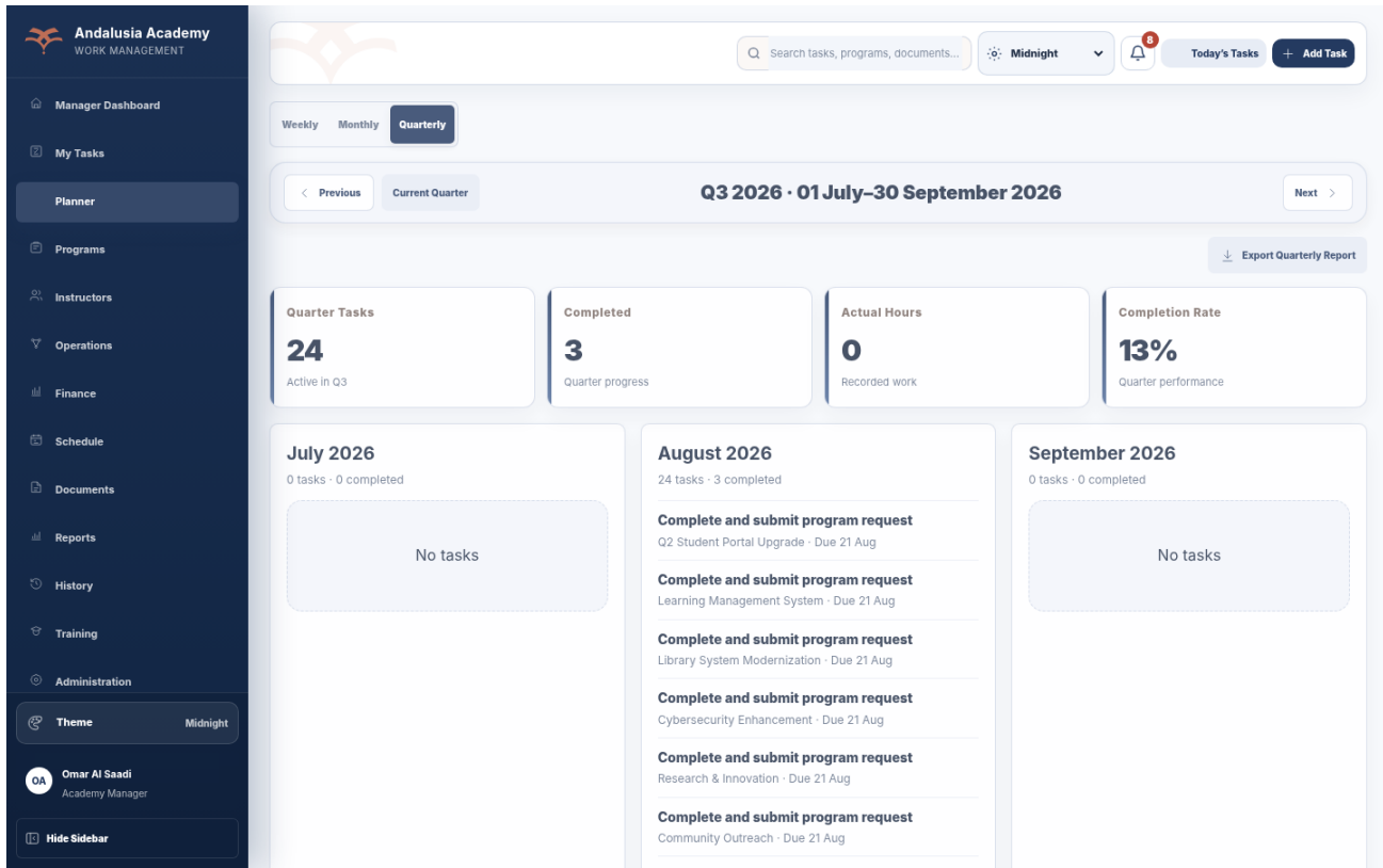
Figure 9 — Quarterly Planner - actual desktop UI
