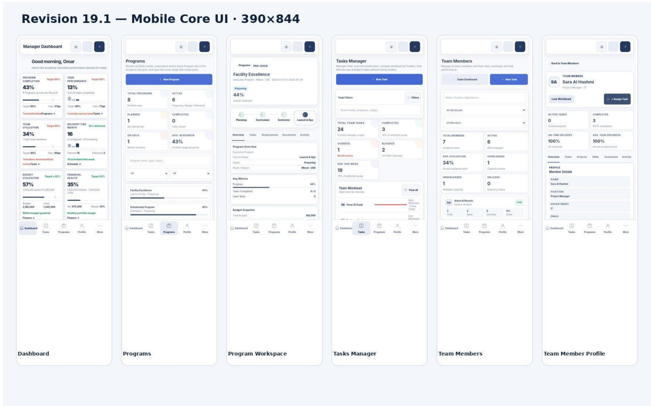
Figure 31 — Core mobile workspace review - Dashboard, Programs, Workspace, Tasks, Team and Team Member Profile
