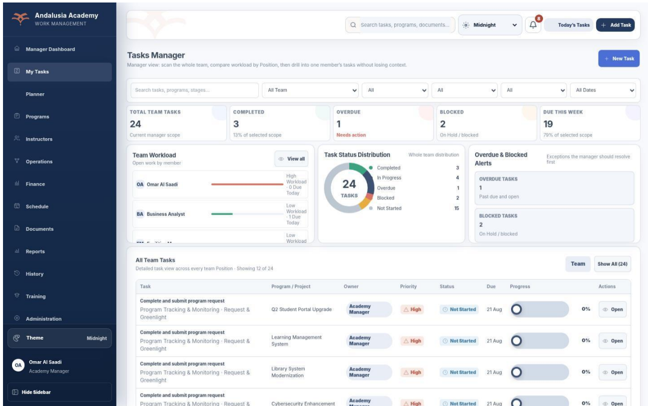
Figure 6 — Tasks / My Tasks - actual desktop UI
