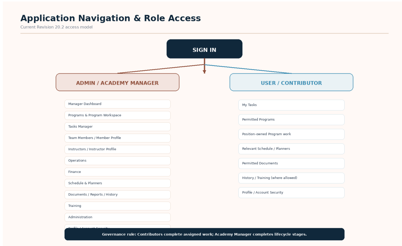
Figure 4 — Role-aware navigation map
