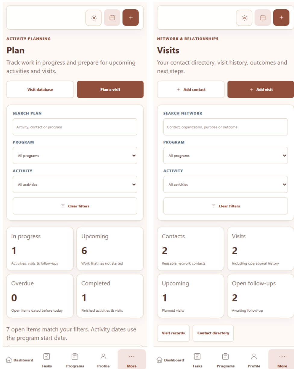
Figures 38 and 39 - Plan and Visits at a 390-pixel mobile viewport, using demonstration records
