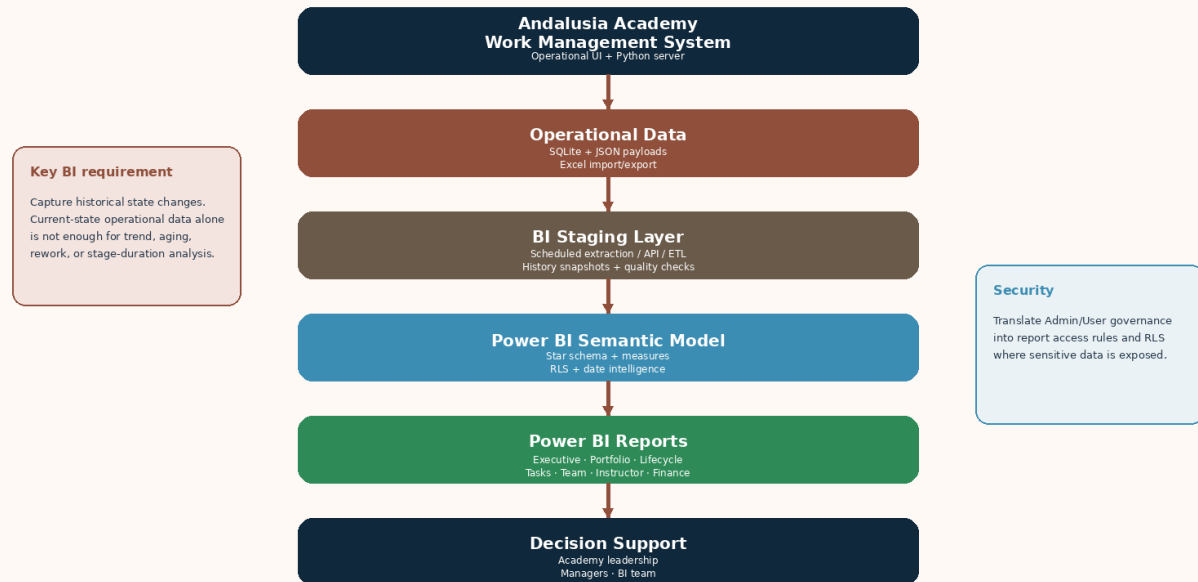
Figure 1 — Recommended operational-to-analytics architecture
