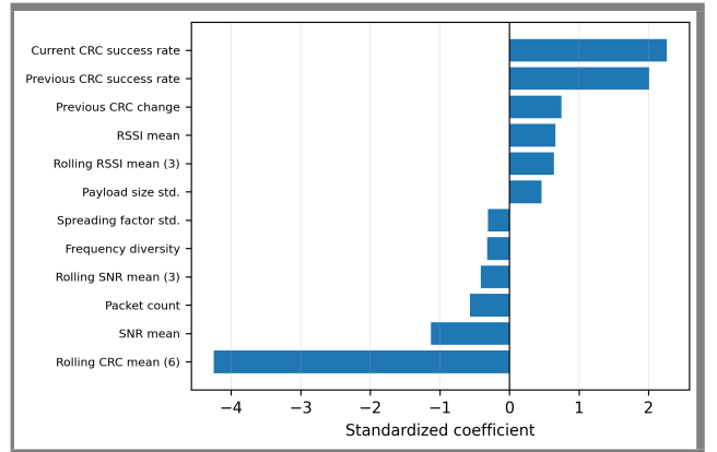
Fig. 3. Largest-magnitude standardized logistic-regression coefficients for \theta = 0.10 . Gateway identifiers are excluded; coefficient magnitude does not establish causal importance.
