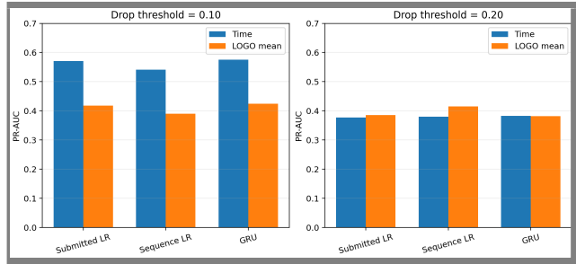
Fig. 7. PR-AUC comparison of the submitted feature-based LR, six-window sequence LR and compact GRU on their common eligible samples.
