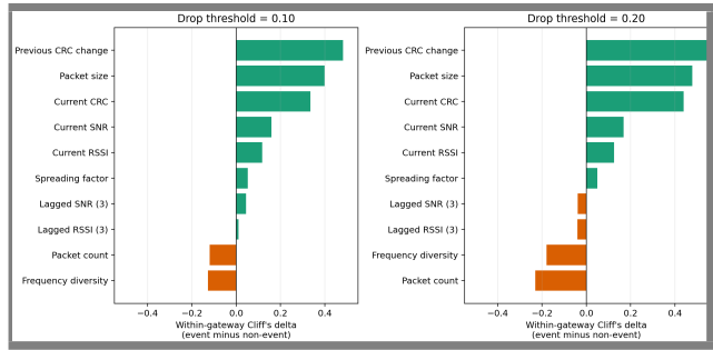
Fig. 6. Within-gateway standardized precursor effects measured with Cliff's delta. The estimates are descriptive associations and do not identify physical causes.
