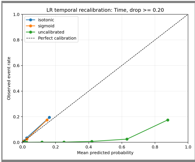
Fig. 5. Chronological reliability diagram for severe degradation before and after leakage-controlled calibration. The dashed diagonal denotes perfect calibration.
