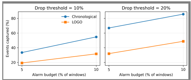
Fig. 2. Degradation events captured at top-risk alarm budgets for time-based and leave-one-gateway-out settings.
