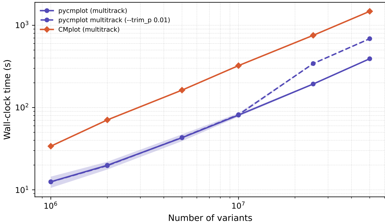
Runtime scaling — Multi-track circular Manhattan plot
