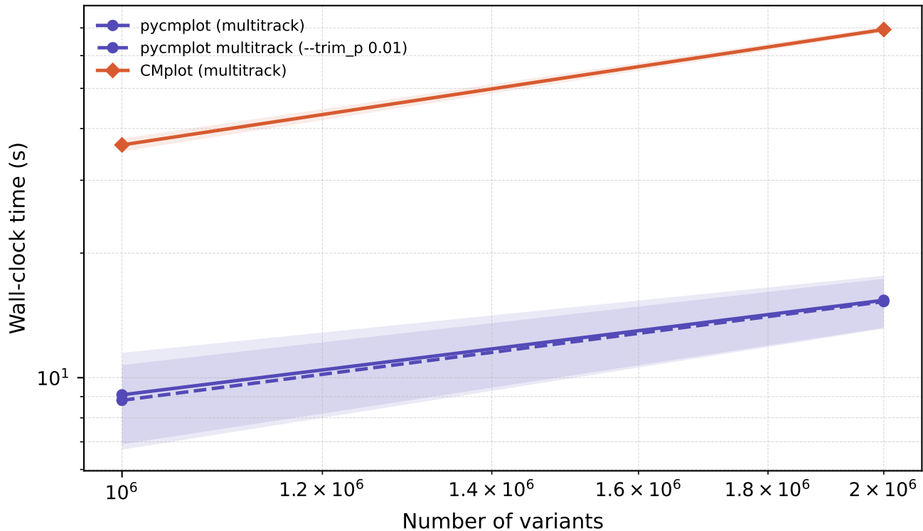
Runtime scaling — Multi-track Manhattan plot
