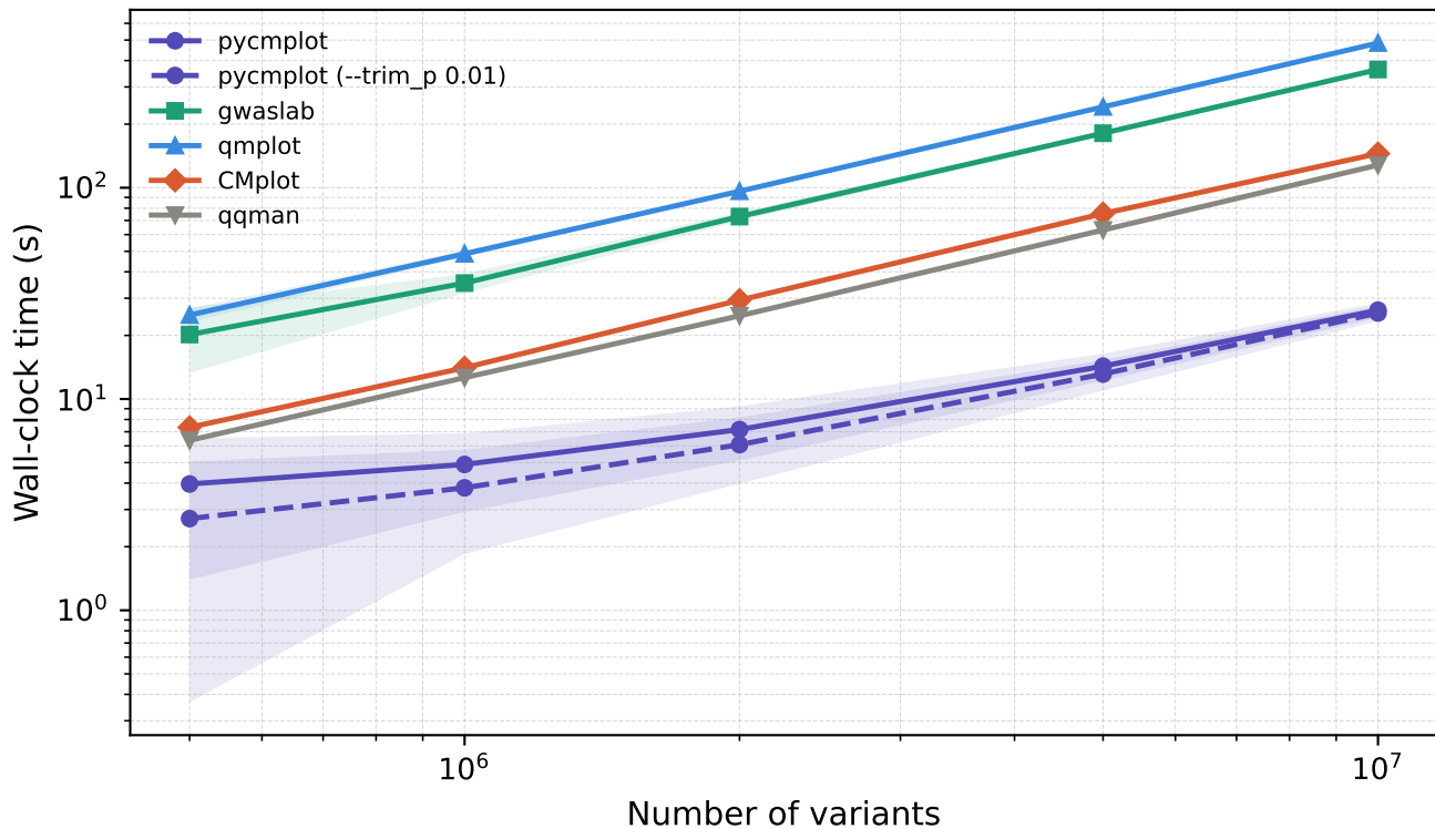
Runtime scaling — Manhattan plot
