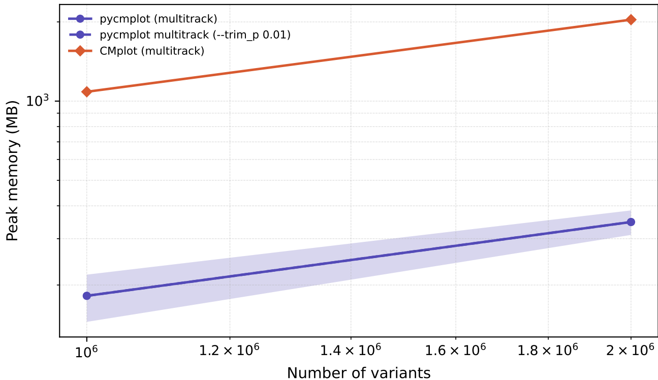
Peak memory scaling — Multi-track Manhattan plot
