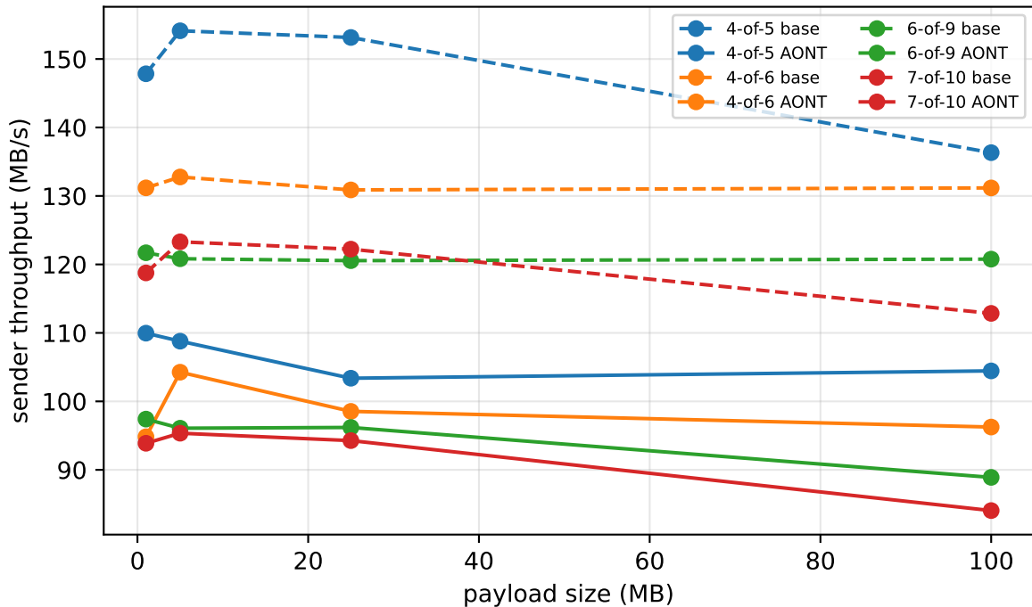
Sender-side throughput vs payload size (solid = AONT-RS, dashed = base)
