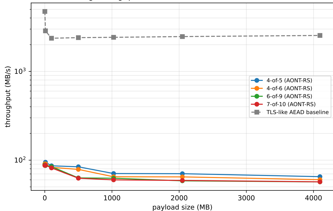
Sealing throughput: BHDAM-R vs a TLS-like AEAD baseline
