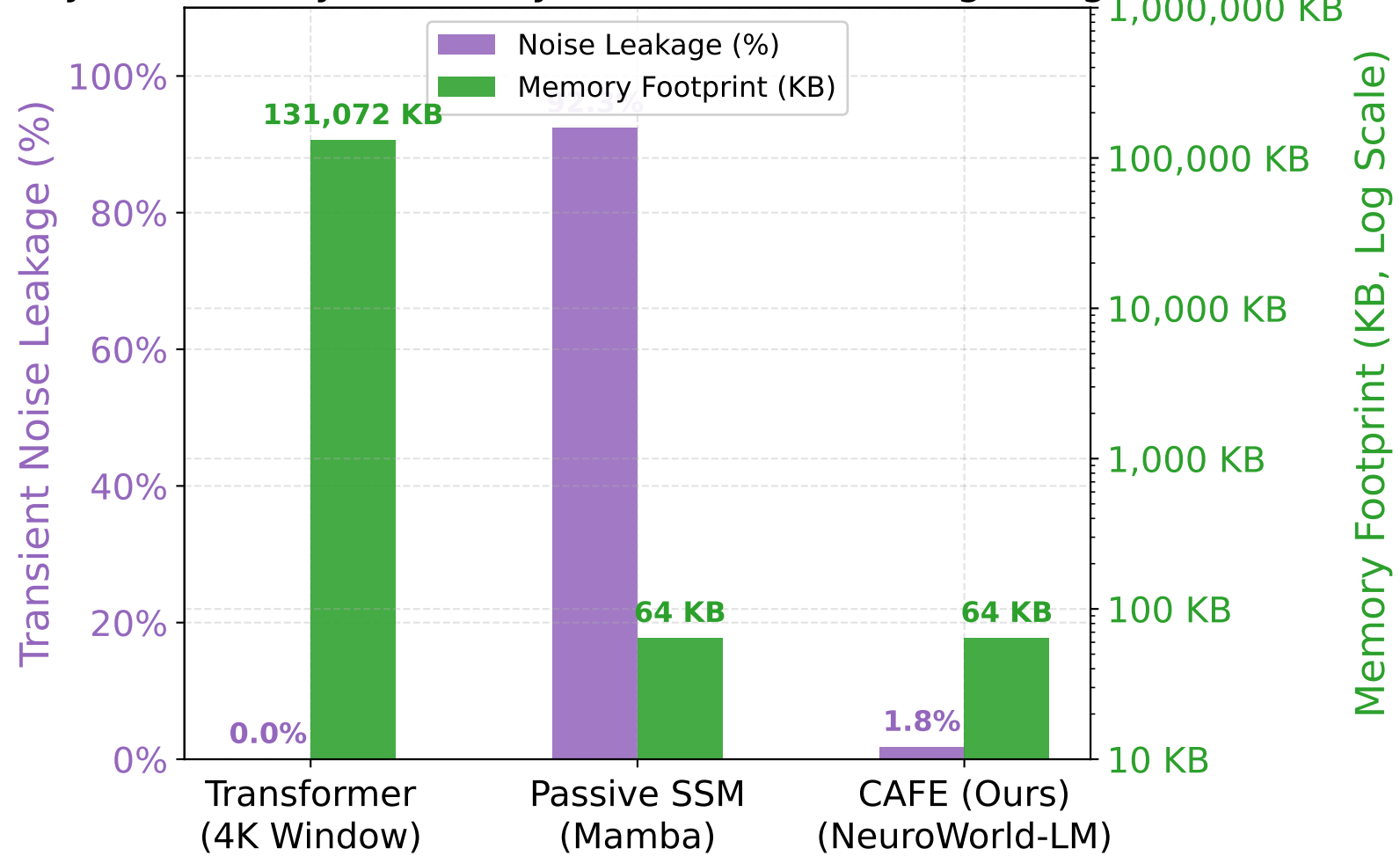
Memory Efficiency &amp; Active Noise Forgetting
