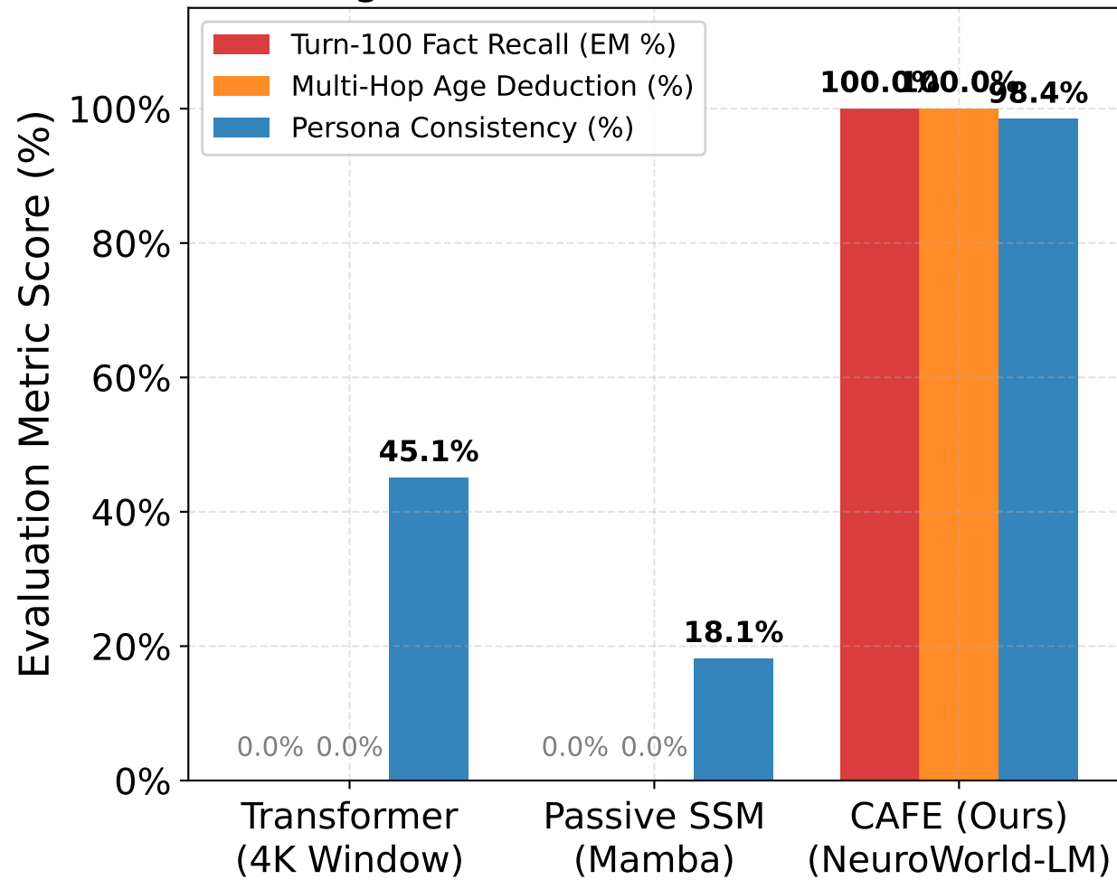
100-Turn Long-Horizon Fact Recall &amp; Persona Stability
