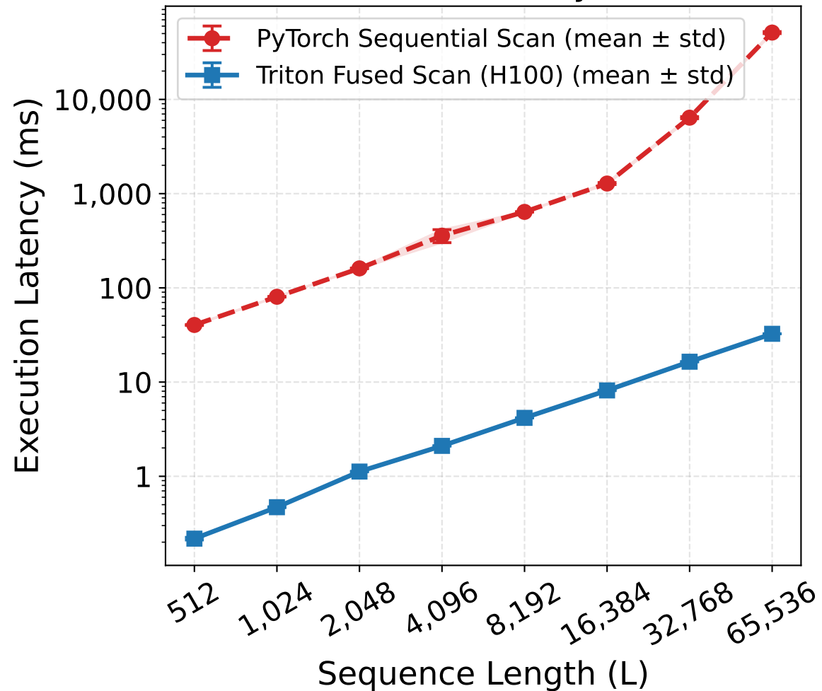
Associative Scan Latency & Deviation
