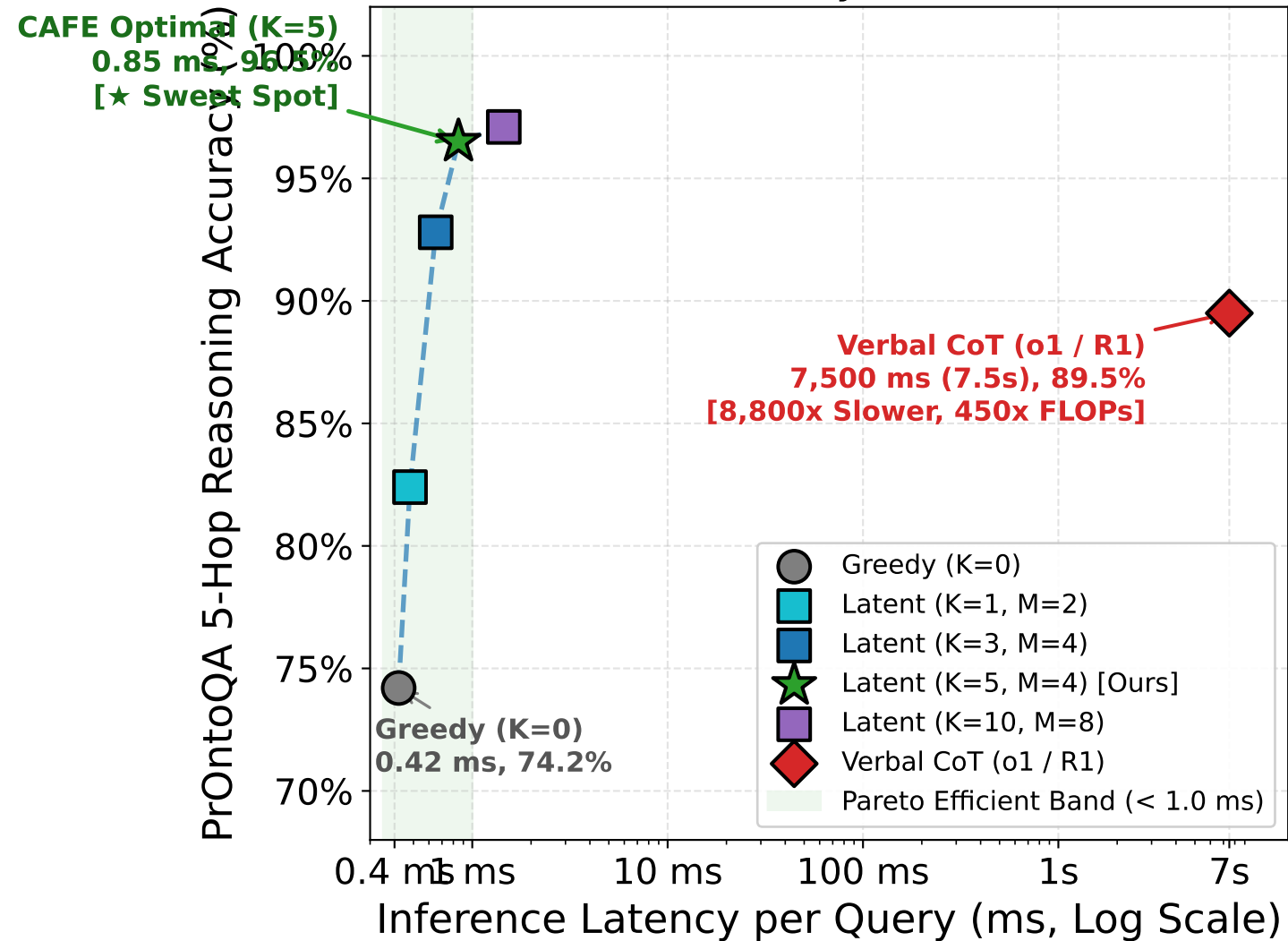
Pareto Frontier: Accuracy vs. Inference Latency
