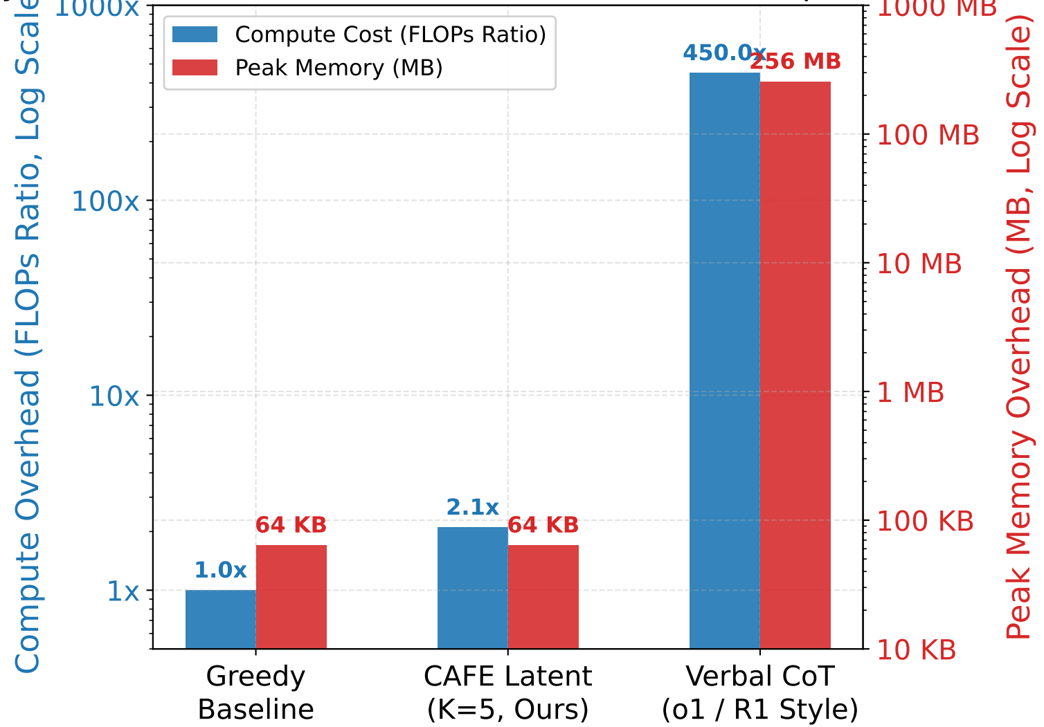
Multi-Dimensional Cost & Resource Footprint
