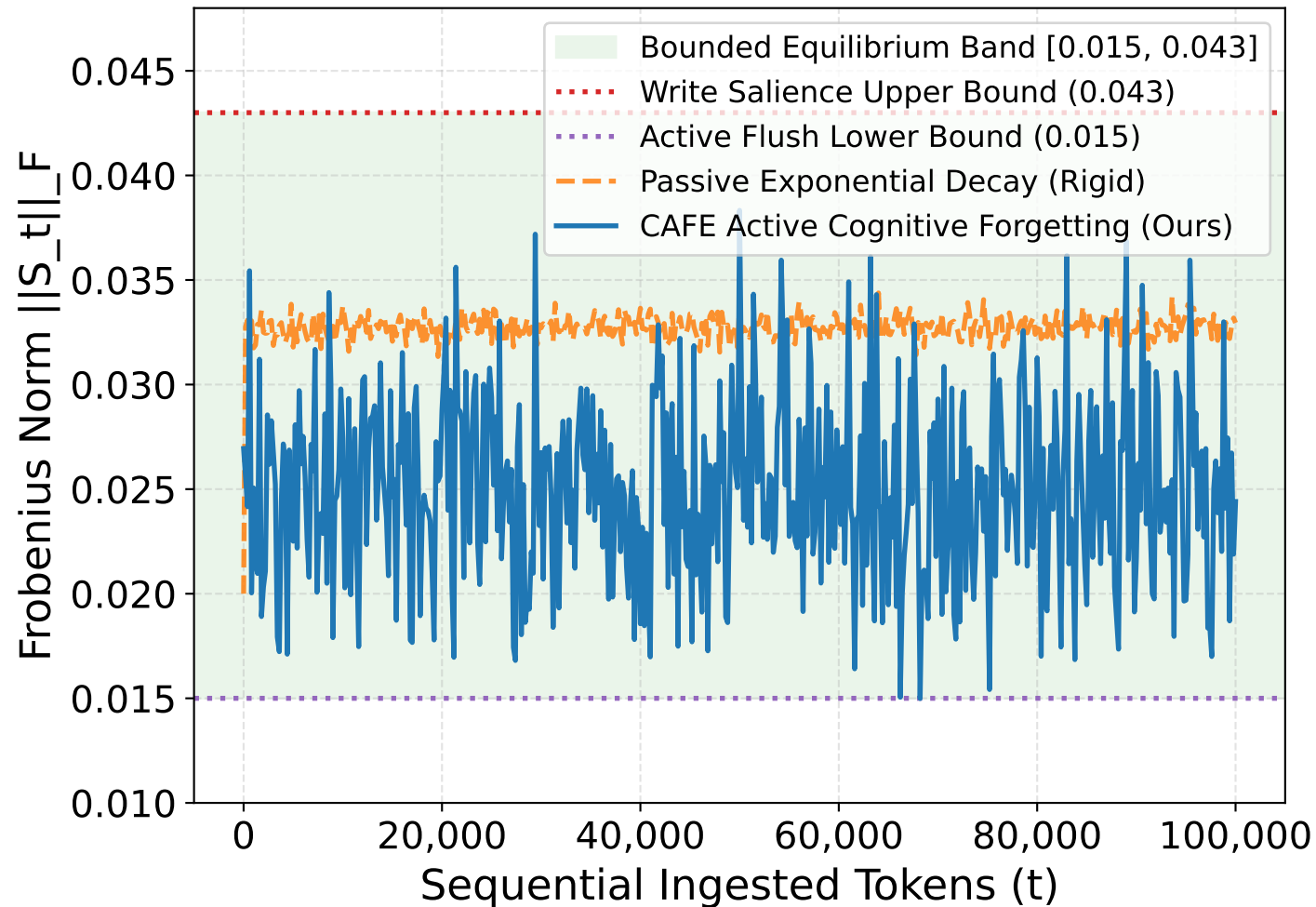
100k-Token State Norm &amp; Boundedness
