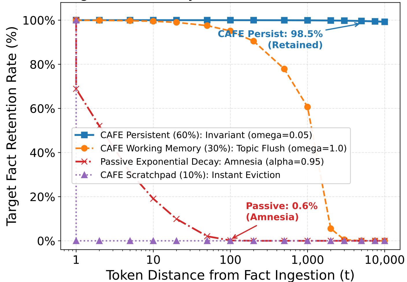
Target Fact Memory Retention vs. Token Distance
