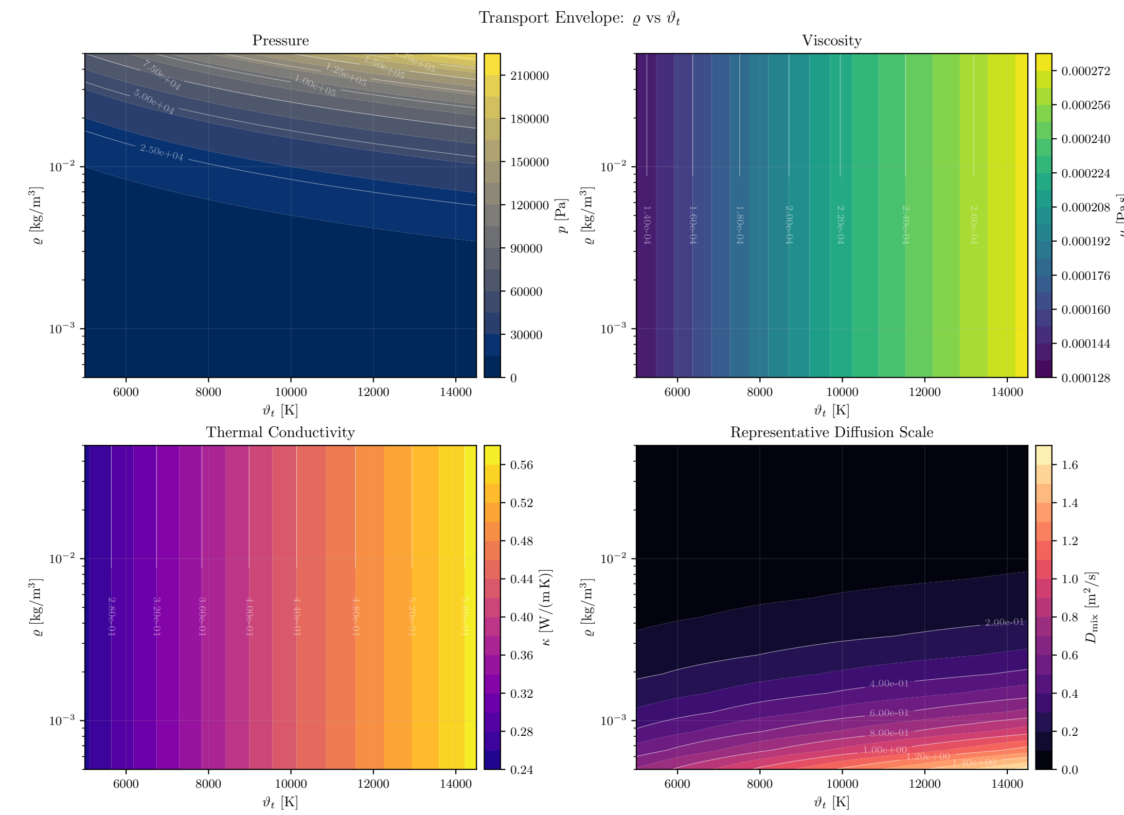
Figure 4. Air5 transport variation with density and translational temperature.
