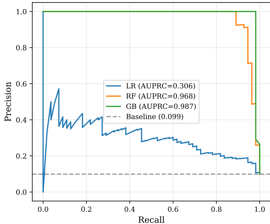
PR — Slurm (all features)
