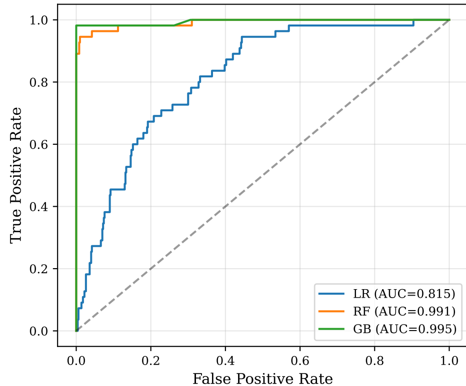
ROC — Slurm (all features)
