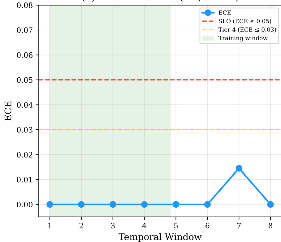
(b) ECE Over Time (GB, Slurm)
