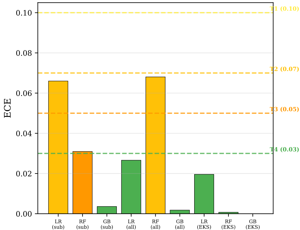
(b) ECE vs Tier Prerequisites
