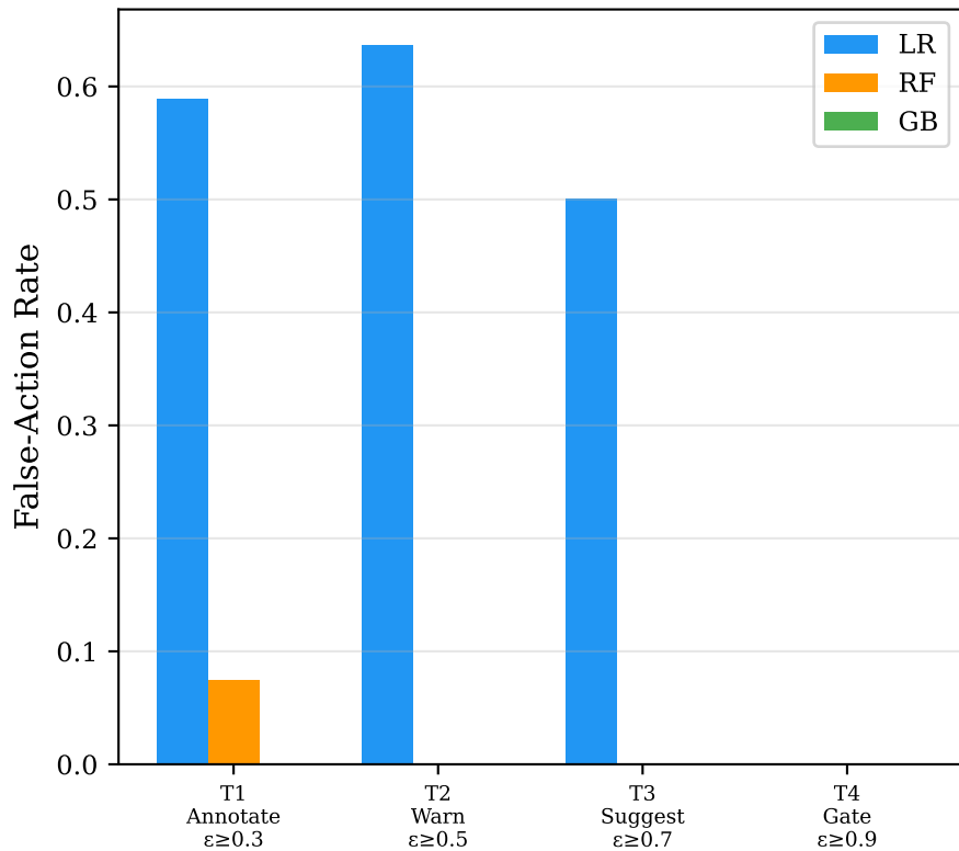
(a) False-Action Rate by Tier (Slurm)
