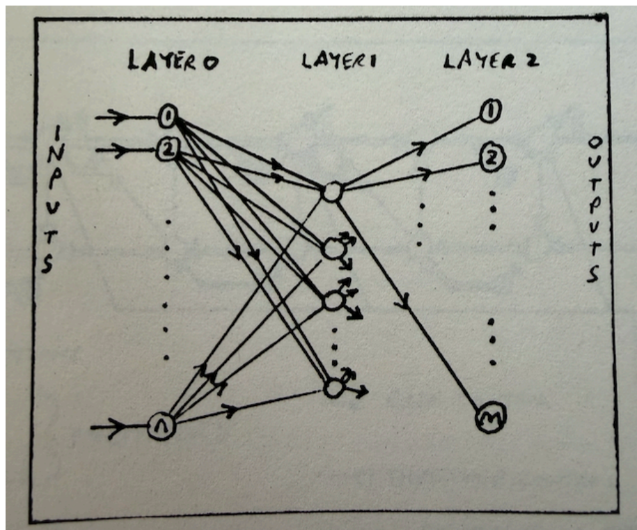
Figure 4: Figure 4: A typical back-propagation network
