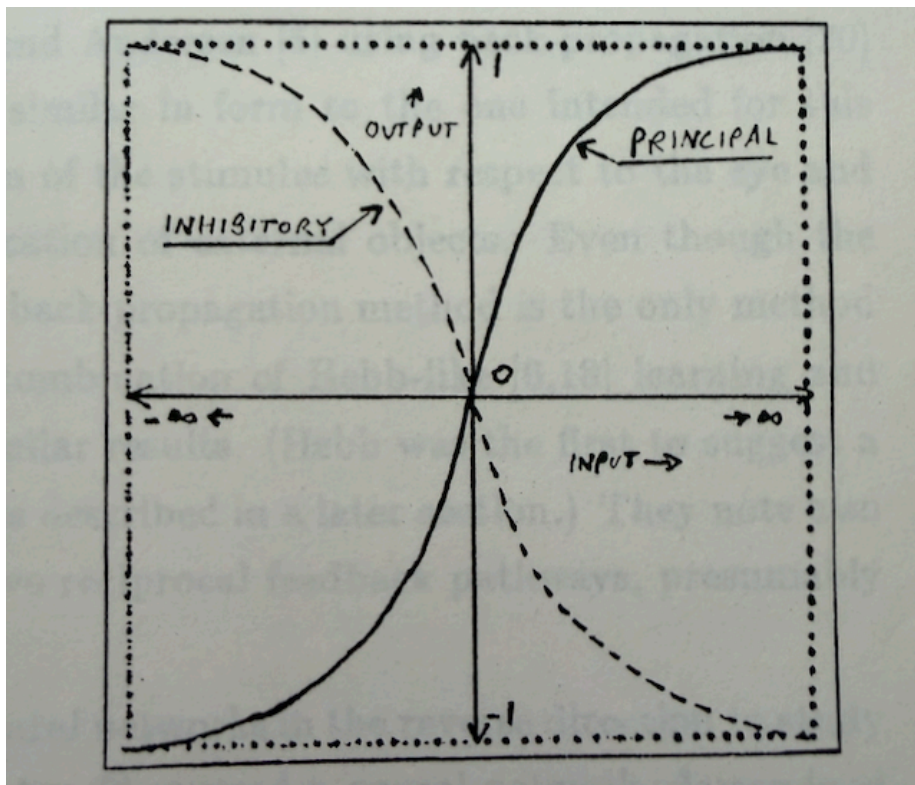
Figure 2: Figure 2: I/O response of simulated neurons
