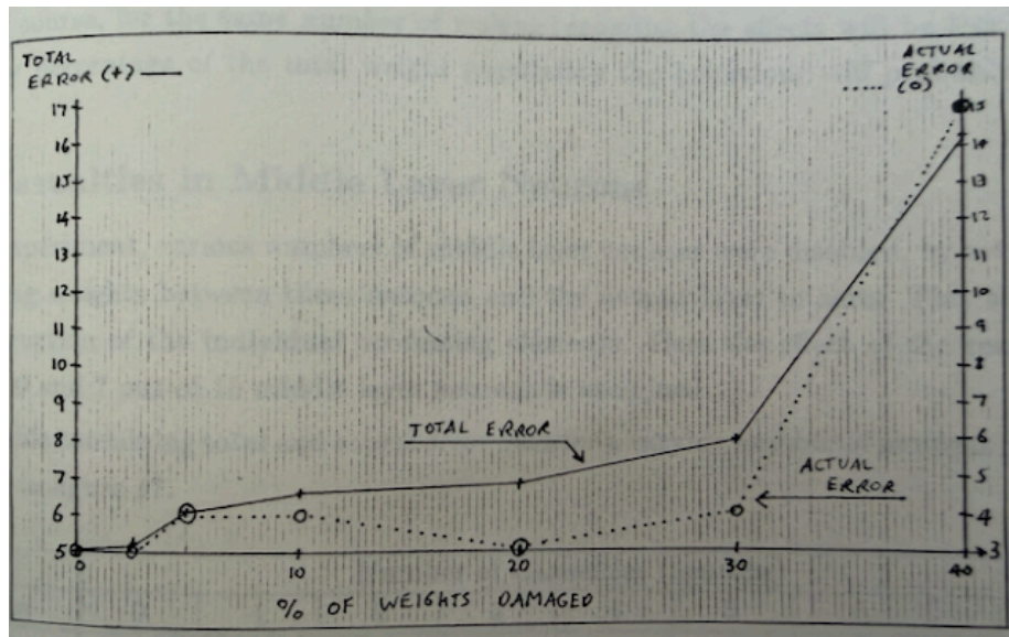
Figure 12: Figure 16: Total and actual error versus % weight casualties
