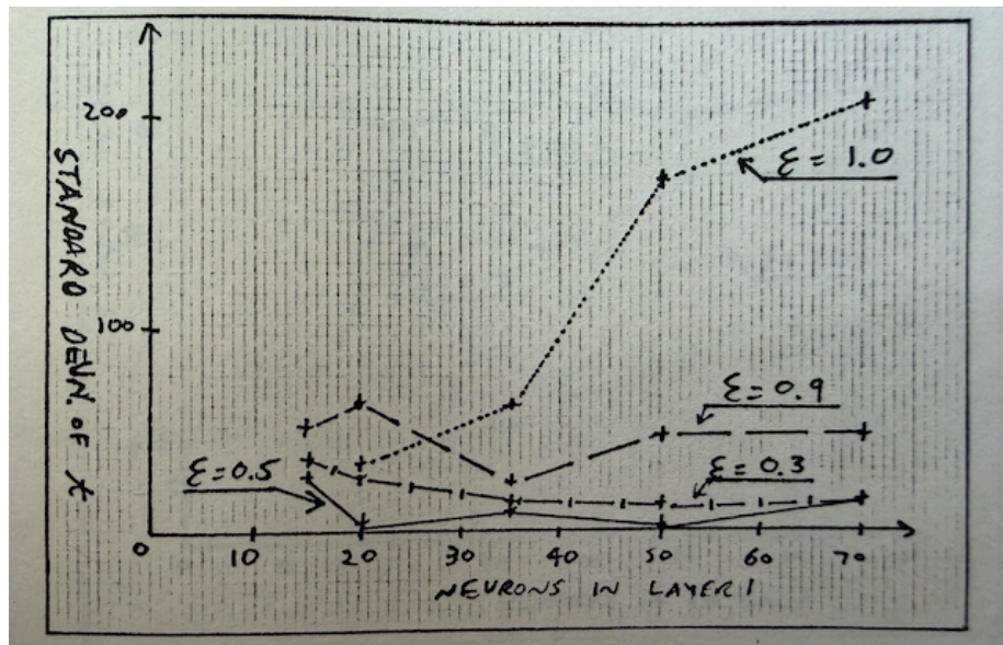
Figure 10: Figure 12: Standard deviation versus number of neurons
