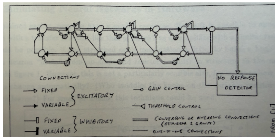
Figure 5: Figure 5: An example of an “improved” neocognitron
