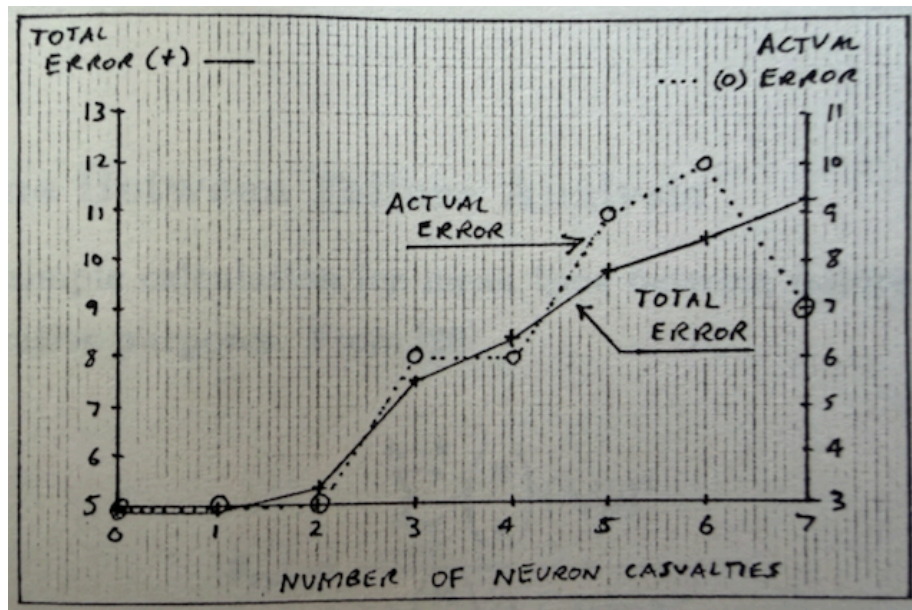
Figure 13: Figure 18: Total and actual errors versus number of layer 1 neuron casualties
