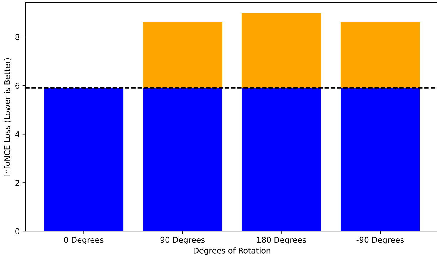
InfoNCE Mutual Information Measurment Between Non-Rotated and Rotated Images
