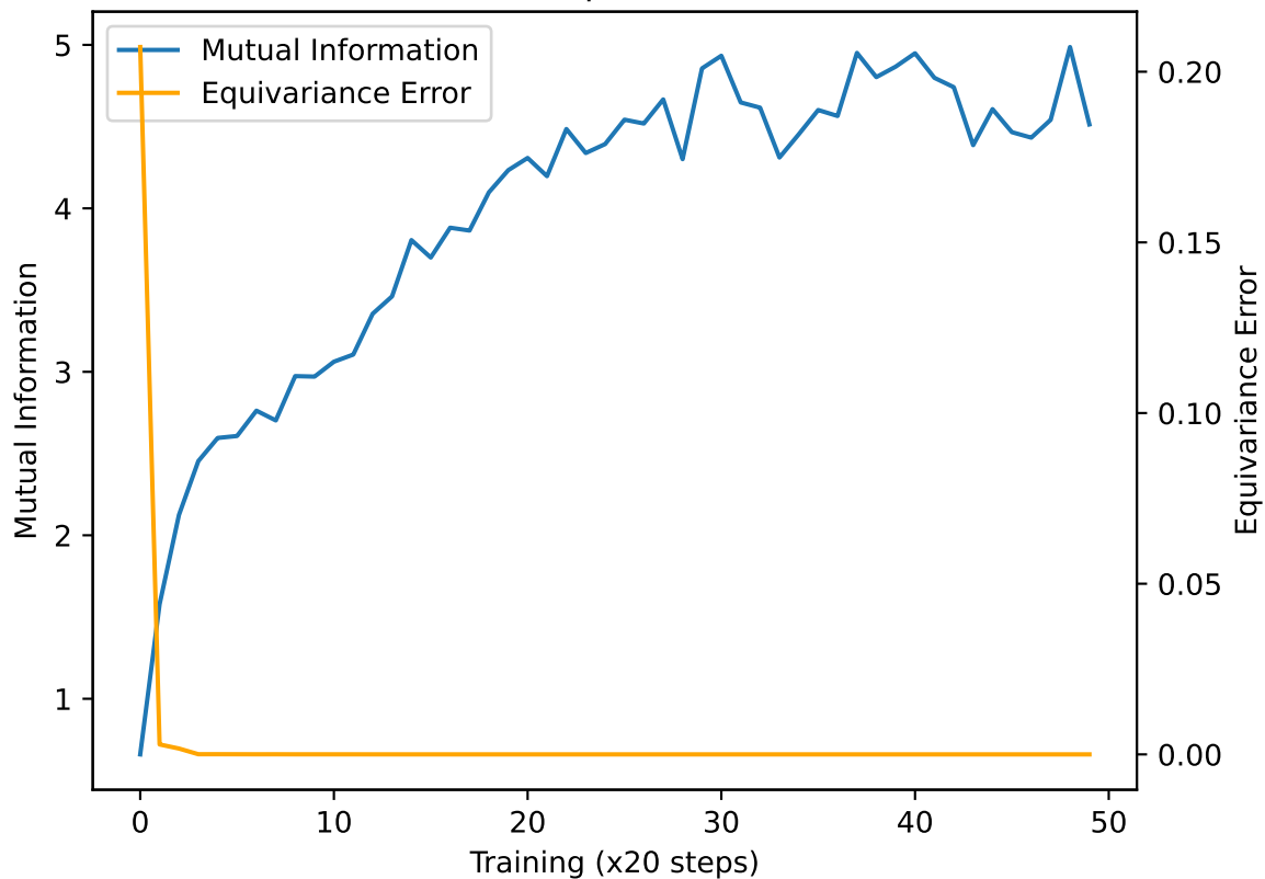
MI increases as equivariance is learned
