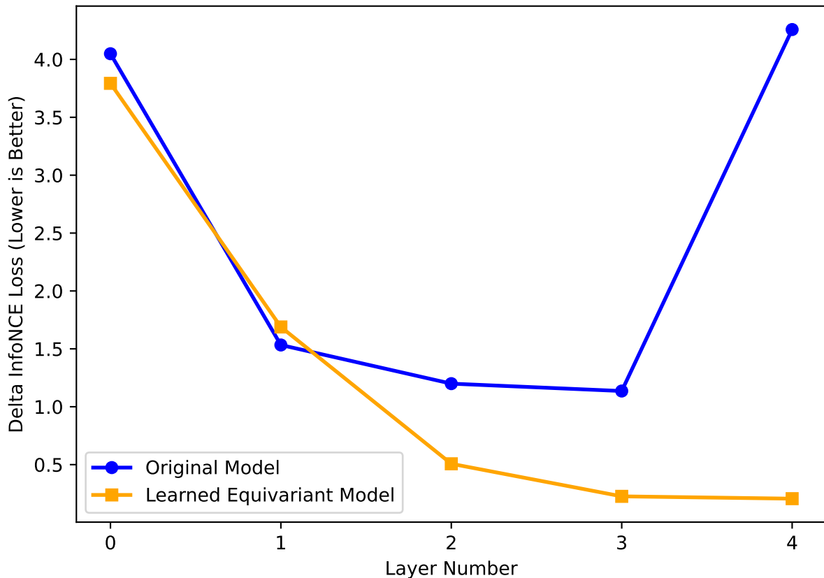
Delta InfoNCE Between Rotated and Non Rotated Images
