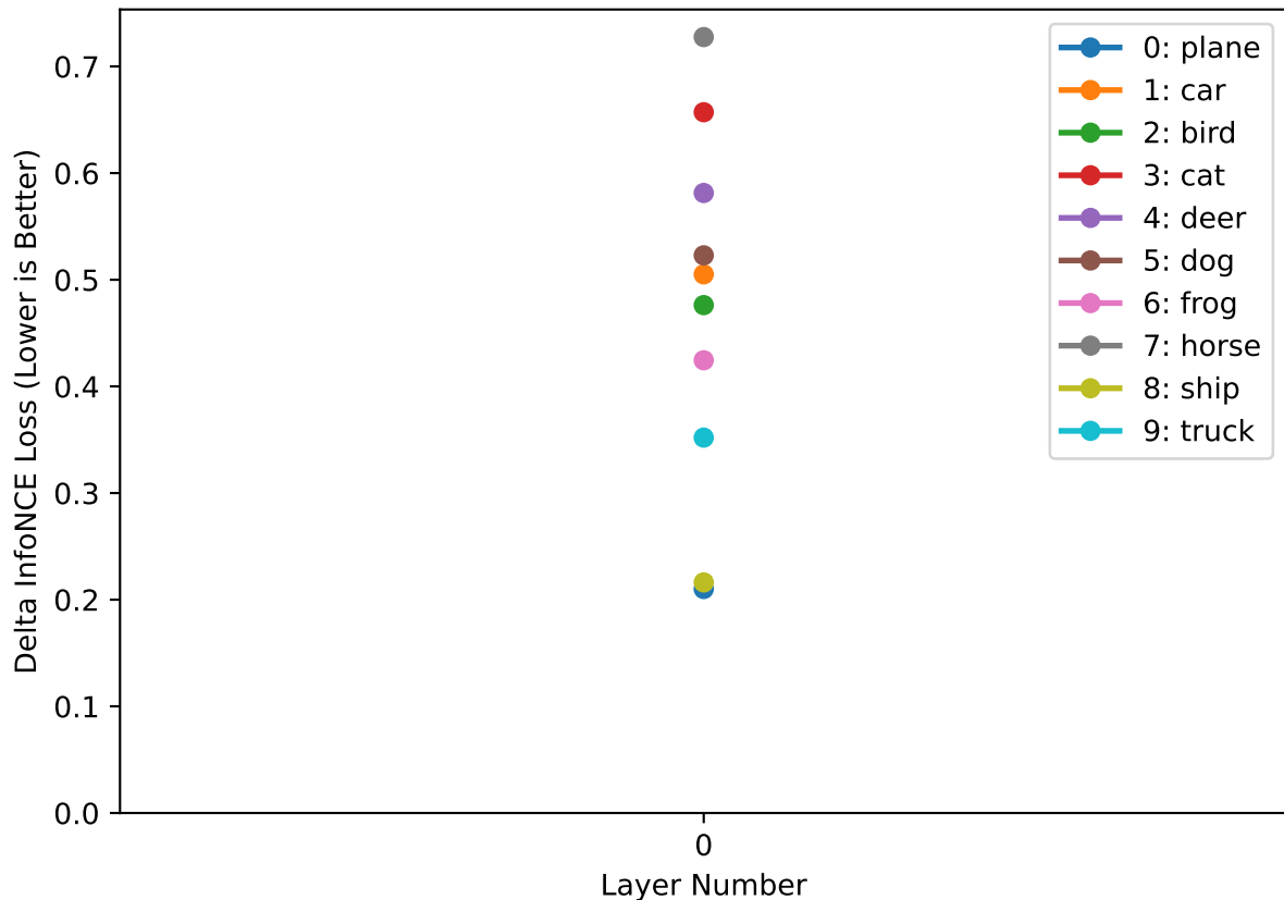
Delta InfoNCE Between Rotated and Non Rotated Images Per Class
