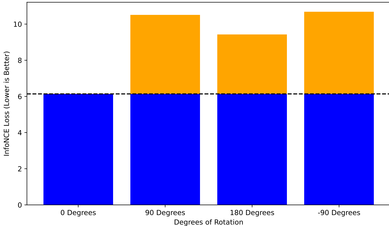
InfoNCE Mutual Information Meausure Between Non-Rotated and Rotated Images
