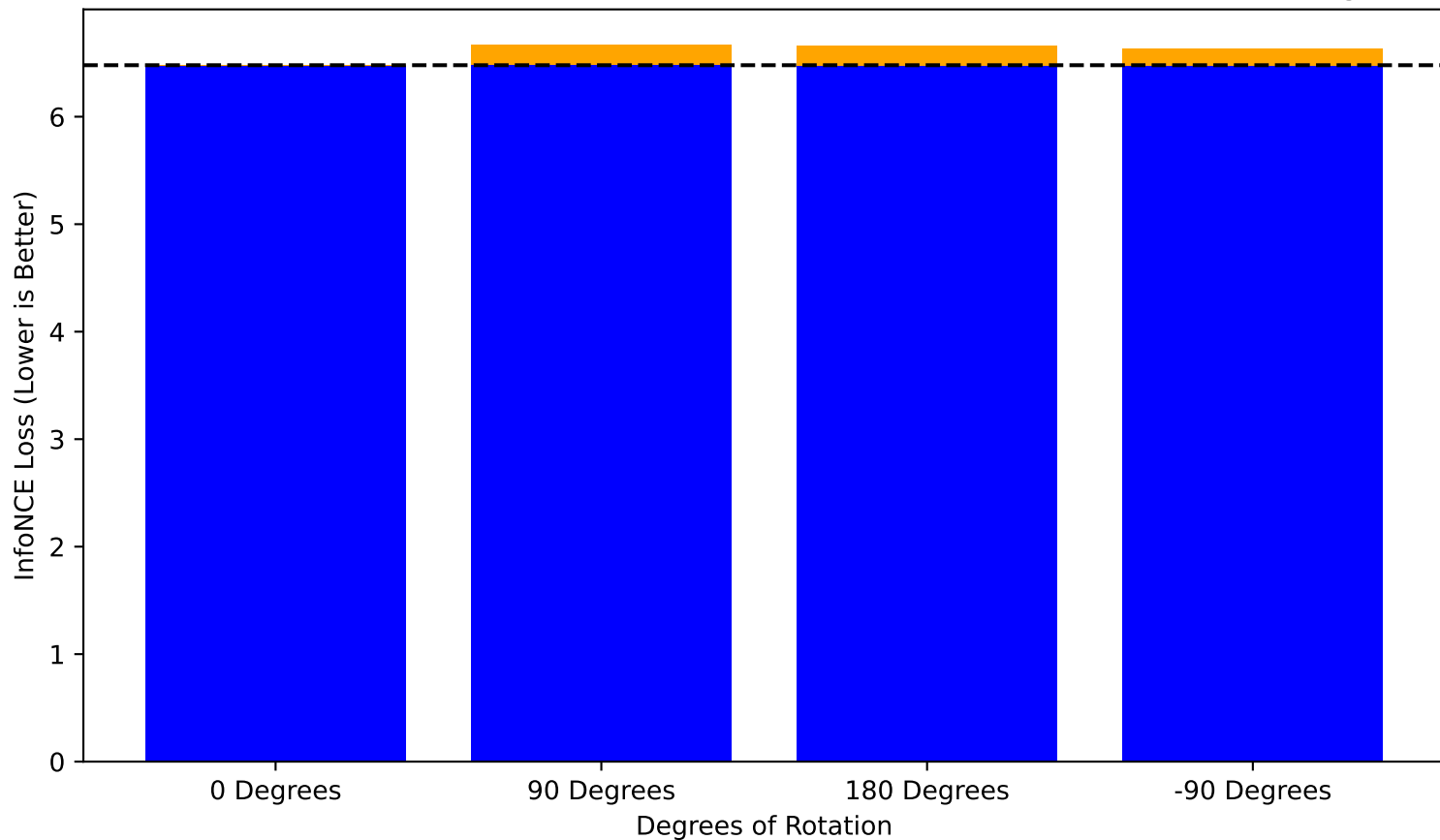
InfoNCE Mutual Information Measure Between Non-Rotated and Rotated Images
