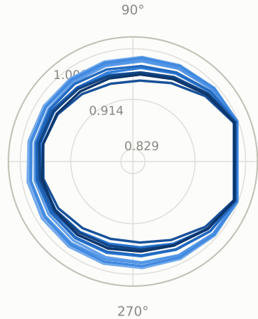
Stress (particles) mlp / anisotropic CKA 0.648-1.000
