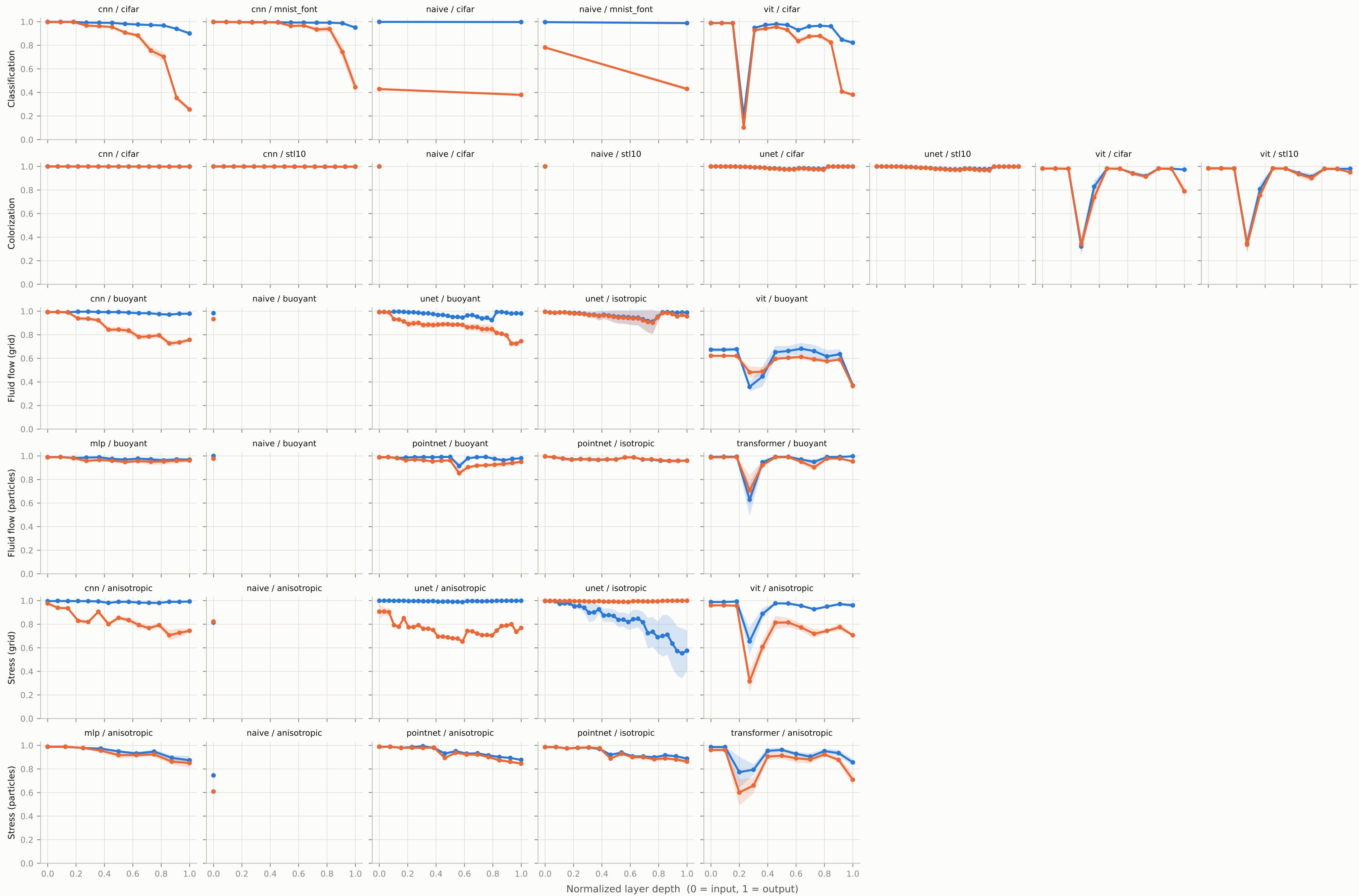
Measured equivariance across depth, at the final epoch mean \pm 1 s.d. over 10 seeds | y: RBF CKA between clean and rotated activations
