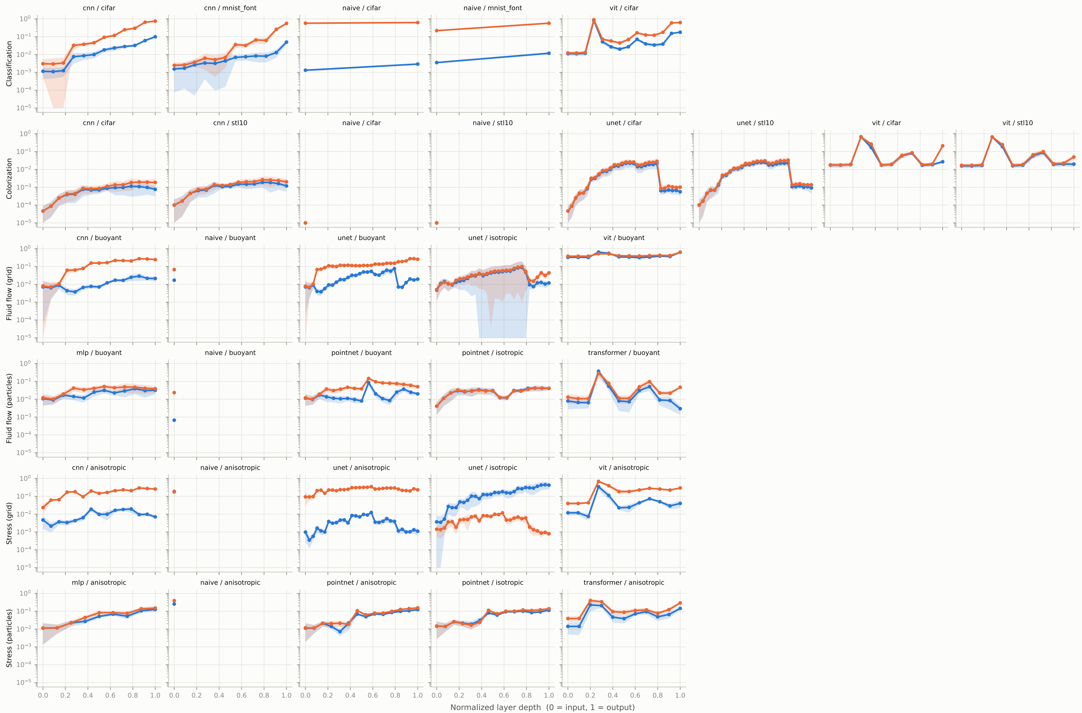
Measured equivariance across depth, at the final epoch \text{mean} \pm 1 \text{ s.d. over } 10 \text{ seeds} | y: equivariance defect 1 - \text{CKA} (log axis)
