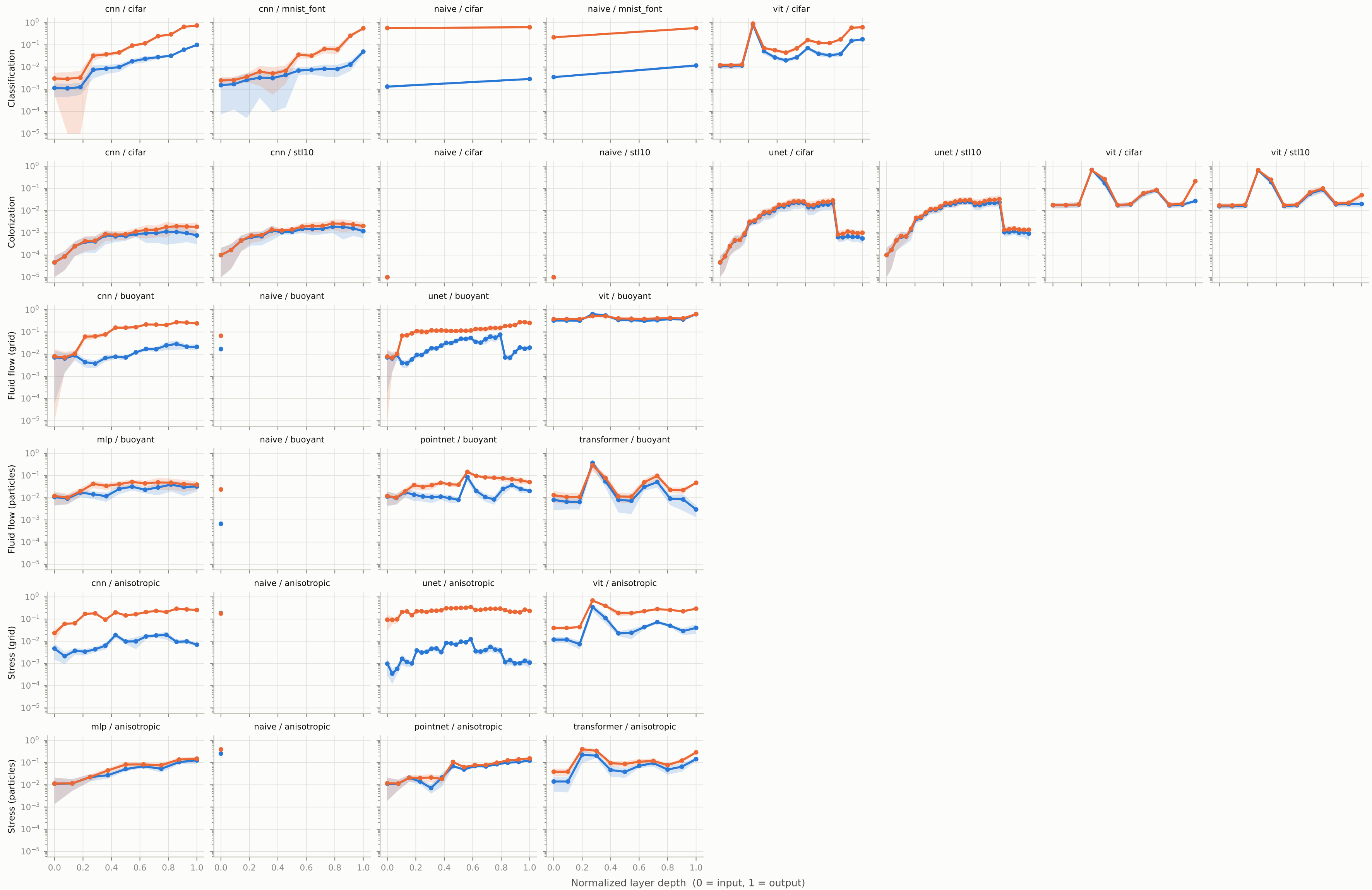
Measured equivariance across depth, at the final epoch mean \pm 1 s.d. over 10 seeds | y: equivariance defect 1 - CKA (log axis) isotropic configs excluded (rotation-symmetric data)
