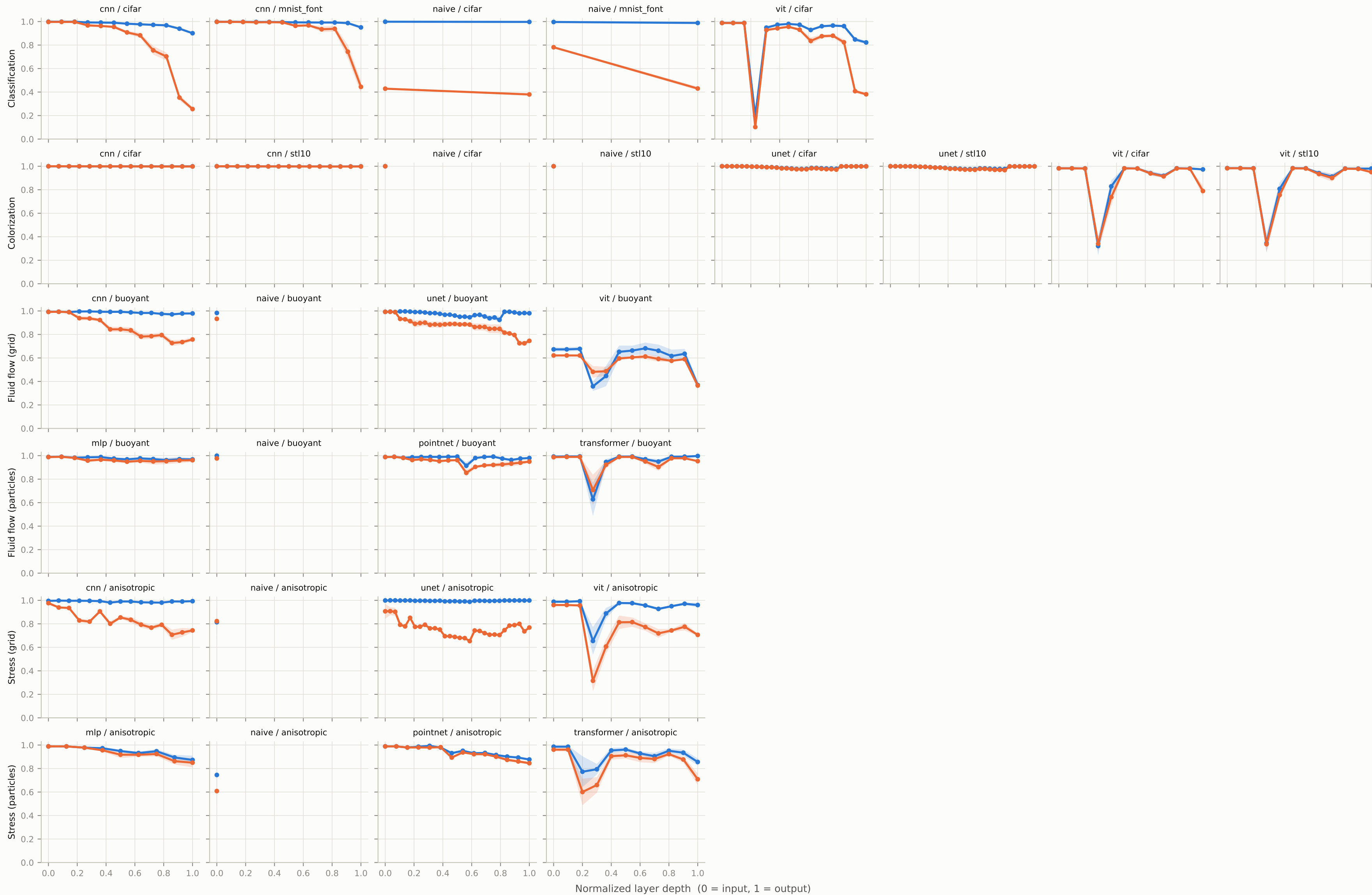
Measured equivariance across depth, at the final epoch mean \pm 1 s.d. over 10 seeds | y: RBF CKA between clean and rotated activations isotropic configs excluded (rotation-symmetric data)
