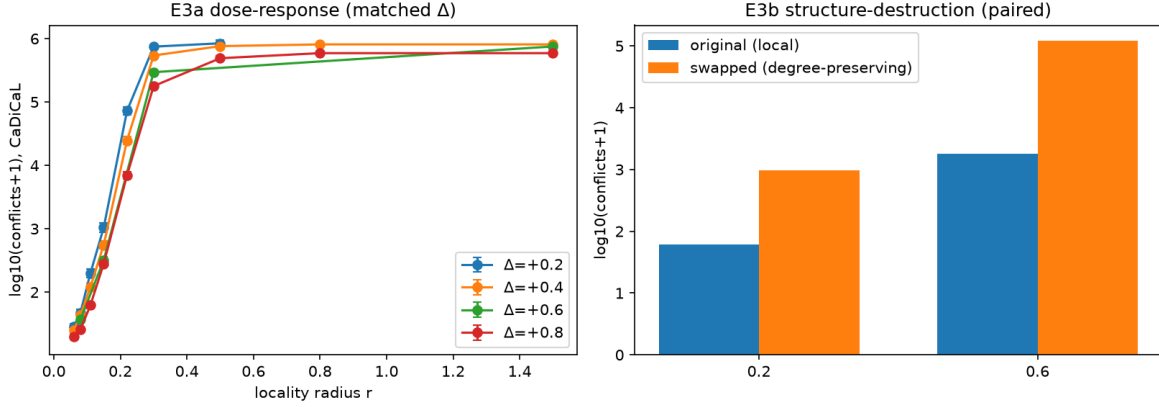
Figure 2: Left: dose-response of difficulty to the locality radius at matched threshold offsets (mean \pm s.e.m., CaDiCaL; \Delta = +0.8 endpoints 1.29 at r=0.06 and 5.77 at r=0.8 ). Right: paired structure-destruction effect (E3b).
