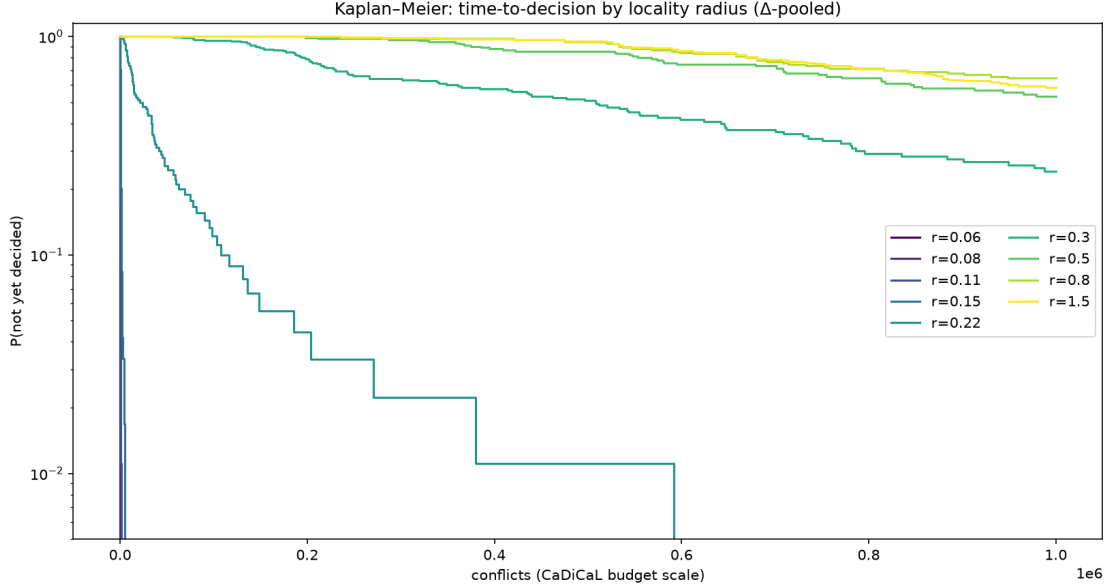
Figure 3: Kaplan–Meier estimates of time-to-decision (conflicts; CaDiCaL, \Delta -pooled). Curves for small r drop to zero within the budget; curves for r \geq 0.5 plateau at high “not yet decided” probability (about a quarter at r = 0.3 ) — the measurability boundary of §5, seen at the solver level.
