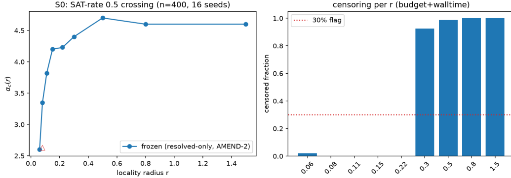
Figure 1: Left: the operational threshold \alpha_c(r) , resolved-only caliber (AMEND-2; \triangle marks radii whose grid has no 0.5-crossing, carried at their lattice-nearest pilot values). Right: censoring fraction per radius (budget + walltime) — the measurability boundary itself tracks r .
