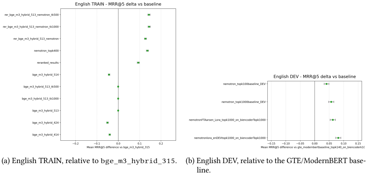
Figure 6: Mean MRR@5 difference versus the reference baseline on the English TRAIN and DEV splits. Error bars show the 95% confidence interval of the paired mean difference.
